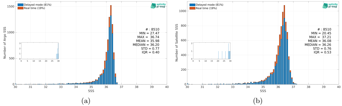
Figure 3: Histograms of SSS from Argo (a) and SMAP SSS L3 v5.3 - 8-Day running (RSS) (b) considering all match-up pairs per bins of 0.1 over the Mississippi river plume Pi-MEP region and for the full satellite product period.
