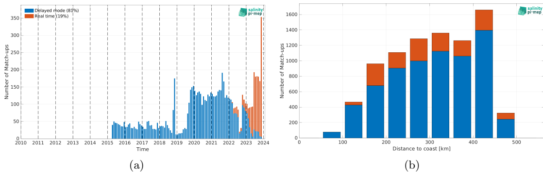
Figure 2: Number of match-ups between Argo and SMAP SSS L3 v5.3 - 8-Day running (RSS) SSS as a function of time (a) and as function of the distance to coast (b) over the Mississippi river plume Pi-MEP region and for the full satellite product period.
