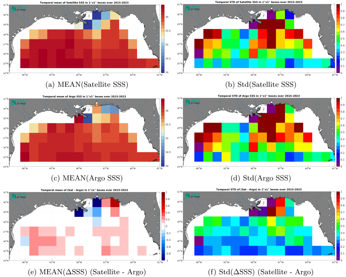
Figure 7: Temporal mean (left) and Std (right) of SSS from SMAP SSS L3 v5.3 - 8-Day running (RSS) (top), Argo (middle), and of \Delta\text{SSS} (Satellite - Argo). Only match-up pairs are used to generate these maps.
