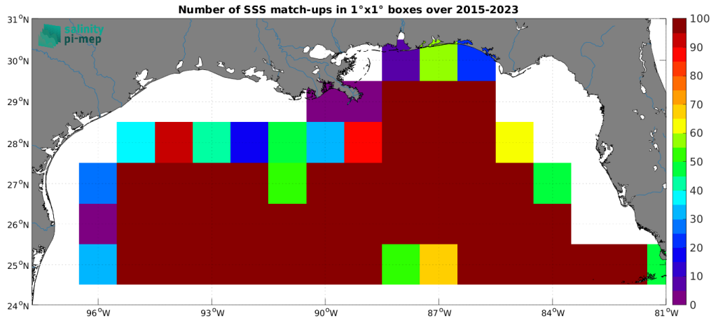
Figure 5: Number of SSS match-ups between Argo SSS and the SMAP SSS L3 v5.3 - 8-Day running (RSS) SSS product for the Mississippi river plume Pi-MEP region over 1^\circ \times 1^\circ boxes and for the full satellite product period.
