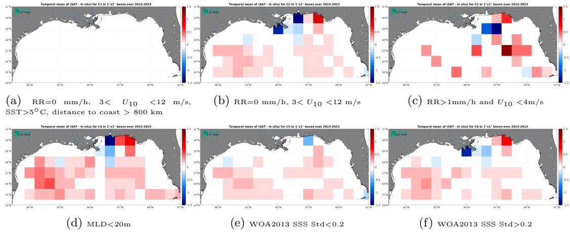
Figure 14: Temporal mean gridded over spatial boxes of size 1^\circ \times 1^\circ of \Delta SSS (SMAP SSS L3 v5.3 - 8-Day running (RSS) - Argo) for 6 different subdatasets corresponding to:RR=0 mm/h, 3 < U_{10} < 12 m/s, SST >5^\circ C, distance to coast > 800 km (a), RR=0 mm/h, 3 < U_{10} < 12 m/s (b), RR >1 mm/h and U_{10} < 4 m/s (c),MLD <20 m (d),WOA2013 SSS Std <0.2 (e),WOA2013 SSS Std >0.2 (f).
