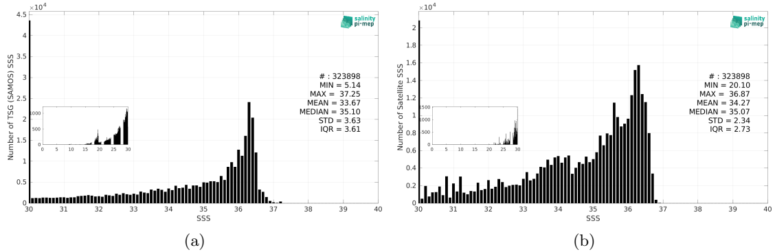
Figure 3: Histograms of SSS from TSG (SAMOS) (a) and SMAP SSS L3 v5.3 - Monthly (RSS) (b) considering all match-up pairs per bins of 0.1 over the Mississippi river plume Pi-MEP region and for the full satellite product period.
