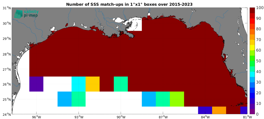
Figure 5: Number of SSS match-ups between TSG (SAMOS) SSS and the SMAP SSS L3 v5.3 - Monthly (RSS) SSS product for the Mississippi river plume Pi-MEP region over 1^\circ \times 1^\circ boxes and for the full satellite product period.
