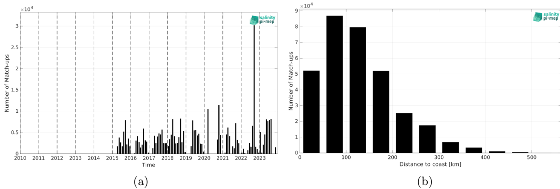
Figure 2: Number of match-ups between TSG (SAMOS) and SMAP SSS L3 v5.3 - Monthly (RSS) SSS as a function of time (a) and as function of the distance to coast (b) over the Mississippi river plume Pi-MEP region and for the full satellite product period.
