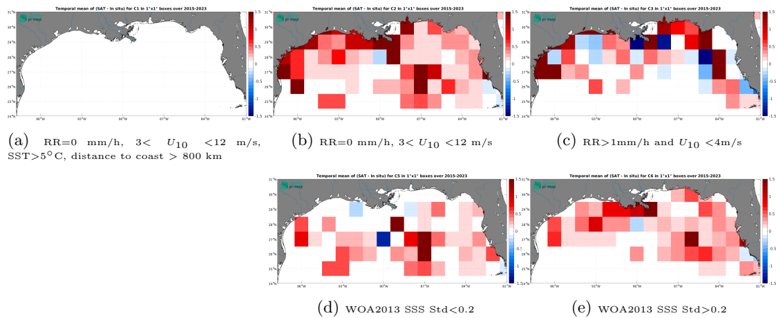
Figure 14: Temporal mean gridded over spatial boxes of size 1^\circ \times 1^\circ of \Delta SSS (SMAP SSS L3 v5.3 - Monthly (RSS) - TSG (SAMOS)) for 5 different subdatasets corresponding to: RR=0 mm/h, 3 < U_{10} < 12 m/s, SST > 5°C, distance to coast > 800 km (a), RR=0 mm/h, 3 < U_{10} < 12 m/s (b), RR > 1mm/h and U_{10} < 4 m/s (c), WOA2013 SSS Std < 0.2 (d), WOA2013 SSS Std > 0.2 (e).
