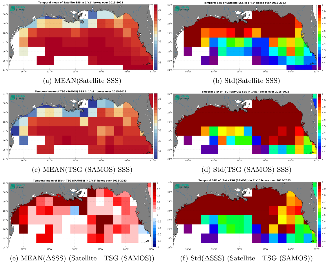
Figure 7: Temporal mean (left) and Std (right) of SSS from SMAP SSS L3 v5.3 - Monthly (RSS) (top), TSG (SAMOS) (middle), and of \Delta\text{SSS} (Satellite - TSG (SAMOS)). Only match-up pairs are used to generate these maps.
