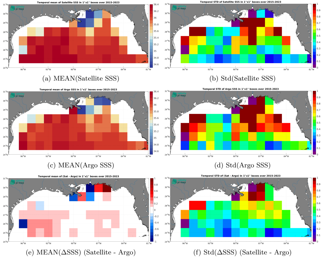
Figure 7: Temporal mean (left) and Std (right) of SSS from SMAP SSS L3 v5.3 - Monthly (RSS) (top), Argo (middle), and of \Delta\text{SSS} (Satellite - Argo). Only match-up pairs are used to generate these maps.
