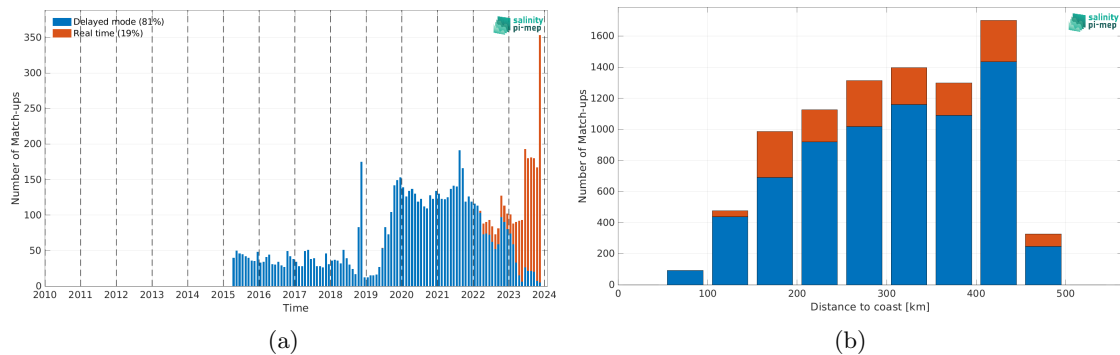
Figure 2: Number of match-ups between Argo and SMAP SSS L3 v5.3 - Monthly (RSS) SSS as a function of time (a) and as function of the distance to coast (b) over the Mississippi river plume Pi-MEP region and for the full satellite product period.
