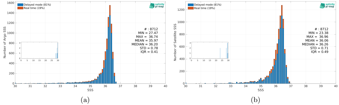
Figure 3: Histograms of SSS from Argo (a) and SMAP SSS L3 v5.3 - Monthly (RSS) (b) considering all match-up pairs per bins of 0.1 over the Mississippi river plume Pi-MEP region and for the full satellite product period.
