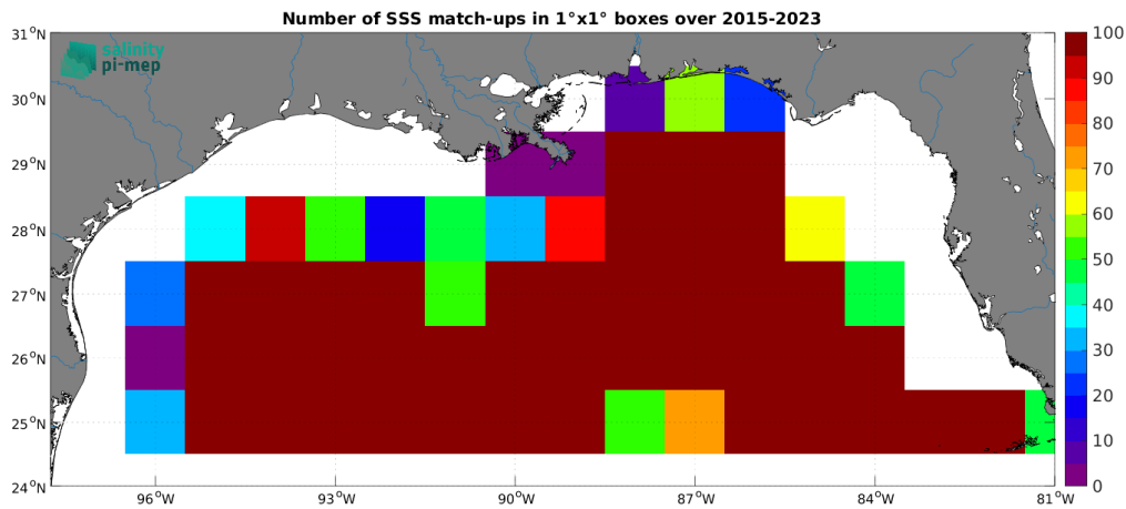
Figure 5: Number of SSS match-ups between Argo SSS and the SMAP SSS L3 v5.3 - Monthly (RSS) SSS product for the Mississippi river plume Pi-MEP region over 1^\circ \times 1^\circ boxes and for the full satellite product period.
