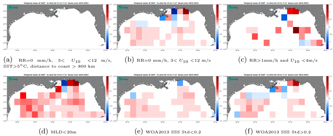
Figure 14: Temporal mean gridded over spatial boxes of size 1^\circ \times 1^\circ of \Delta SSS (SMAP SSS L3 v5.3 - Monthly (RSS) - Argo) for 6 different subdatasets corresponding to:RR=0 mm/h, 3 < U_{10} < 12 m/s, SST > 5^\circ\text{C} , distance to coast > 800 km (a), RR=0 mm/h, 3 < U_{10} < 12 m/s (b), RR > 1 mm/h and U_{10} < 4 m/s (c),MLD < 20 m (d),WOA2013 SSS Std < 0.2 (e),WOA2013 SSS Std > 0.2 (f).
