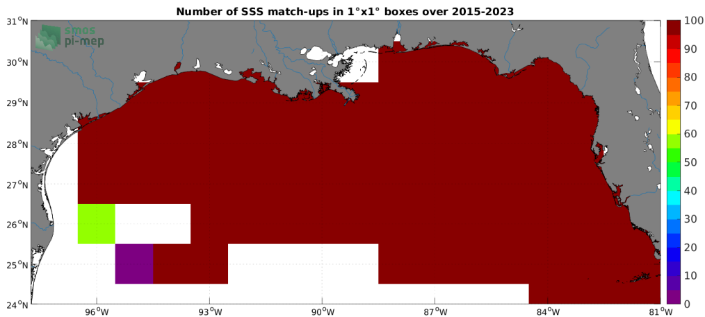
Figure 4: Number of SSS match-ups between TSG (SAMOS) SSS and the SMAP SSS L3 v5 - Monthly (RSS) SSS product for the Mississippi river plume Pi-MEP region over 1^\circ \times 1^\circ boxes and for the full satellite product period.
