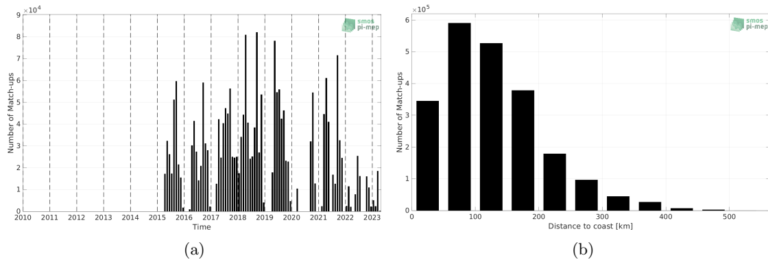
Figure 1: Number of match-ups between TSG (SAMOS) and SMAP SSS L3 v5 - Monthly (RSS) SSS as a function of time (a) and as function of the distance to coast (b) over the Mississippi river plume Pi-MEP region and for the full satellite product period.
