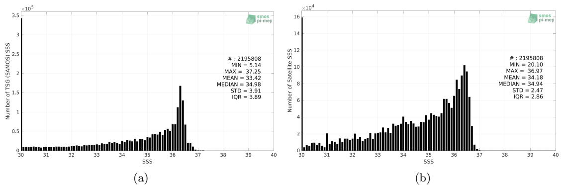
Figure 2: Histograms of SSS from TSG (SAMOS) (a) and SMAP SSS L3 v5 - Monthly (RSS) (b) considering all match-up pairs per bins of 0.1 over the Mississippi river plume Pi-MEP region and for the full satellite product period.
