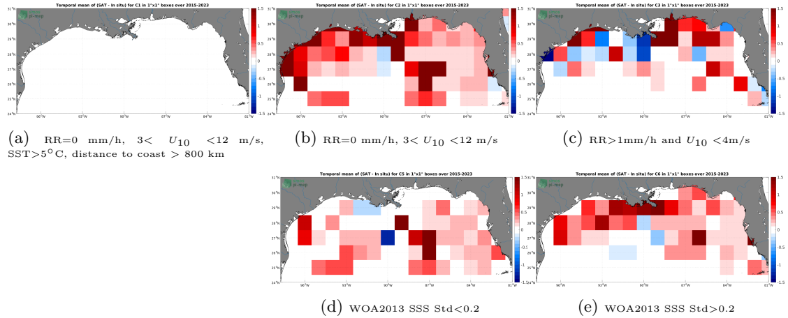
Figure 12: Temporal mean gridded over spatial boxes of size 1^{\circ}\times 1^{\circ} of \Delta\text{SSS} (SMAP SSS L3 v5 - Monthly (RSS) - TSG (SAMOS)) for 5 different subdatasets corresponding to:RR=0 mm/h, 3 < U_{10} < 12 m/s, SST > 5^{\circ}\text{C} , distance to coast > 800 km (a), RR=0 mm/h, 3 < U_{10} < 12 m/s (b), RR > 1 mm/h and U_{10} < 4 m/s (c), WOA2013 SSS Std < 0.2 (d), WOA2013 SSS Std > 0.2 (e).
