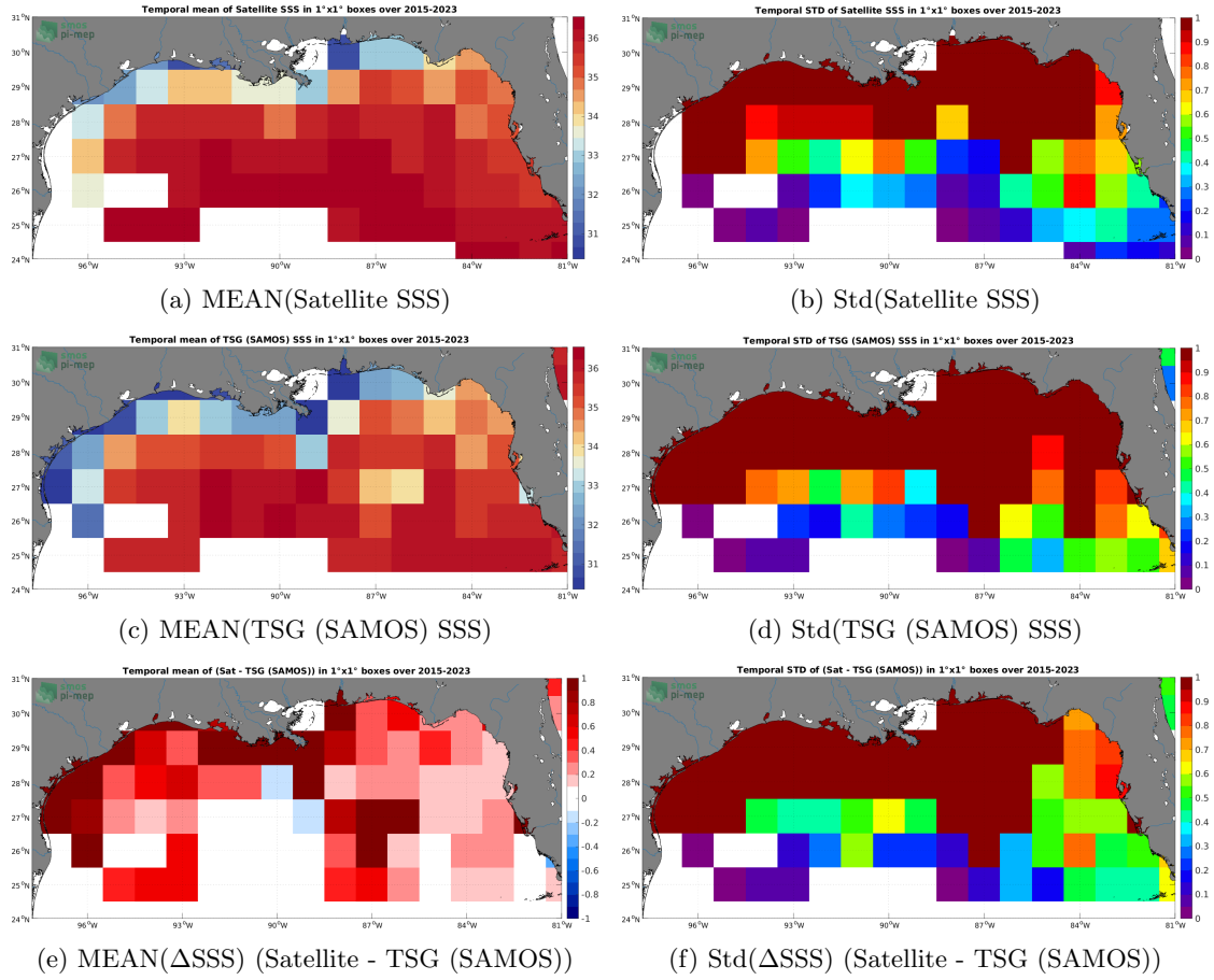
Figure 6: Temporal mean (left) and Std (right) of SSS from SMAP SSS L3 v5 - Monthly (RSS) (top), TSG (SAMOS) (middle), and of \Delta SSS (Satellite - TSG (SAMOS)). Only match-up pairs are used to generate these maps.
