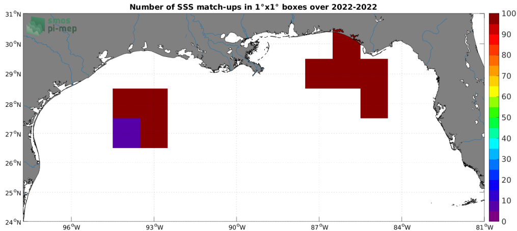
Figure 4: Number of SSS match-ups between Saildrone SSS and the SMAP SSS L3 v5 - Monthly (RSS) SSS product for the Mississippi river plume Pi-MEP region over 1^\circ \times 1^\circ boxes and for the full satellite product period.
