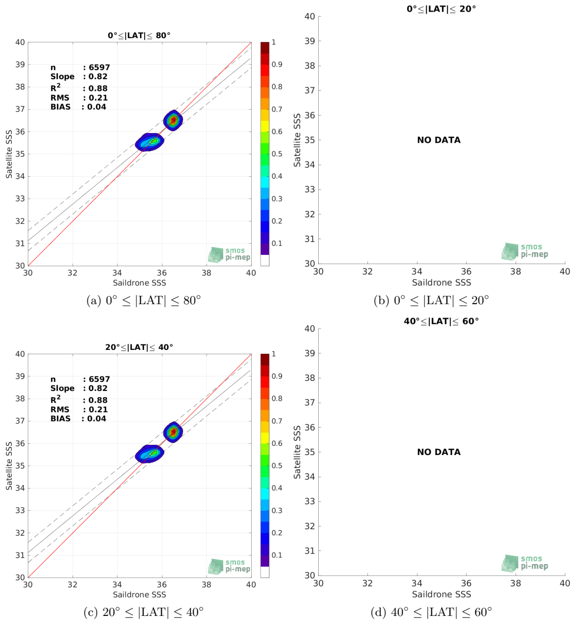
Figure 9: Contour maps of the concentration of SMAP SSS L3 v5 - Monthly (RSS) SSS (y-axis) versus Saïldrone SSS (x-axis) at match-up pairs for different latitude bands. For each plot, the red line shows x=y . The black thin and dashed lines indicate a linear fit through the data cloud and the \pm 95\% confidence levels, respectively. The number match-up pairs n , the slope and R^2 coefficient of the linear fit, the root mean square (RMS) and the mean bias between satellite and in situ data are indicated for each latitude band in each plots.
