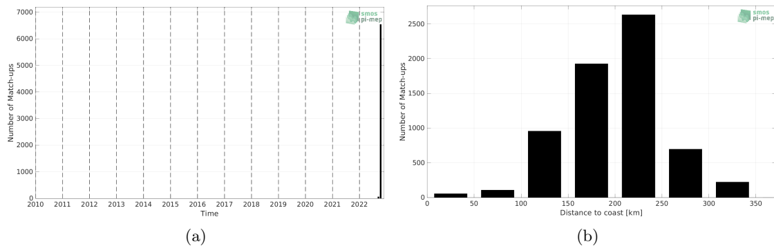
Figure 1: Number of match-ups between Sairdrone and SMAP SSS L3 v5 - Monthly (RSS) SSS as a function of time (a) and as function of the distance to coast (b) over the Mississippi river plume Pi-MEP region and for the full satellite product period.
