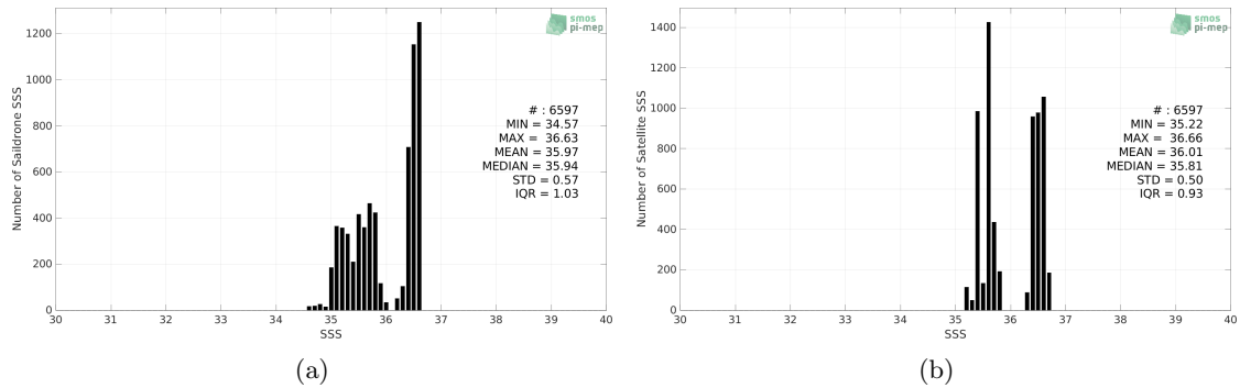
Figure 2: Histograms of SSS from Sailldrone (a) and SMAP SSS L3 v5 - Monthly (RSS) (b) considering all match-up pairs per bins of 0.1 over the Mississippi river plume Pi-MEP region and for the full satellite product period.
