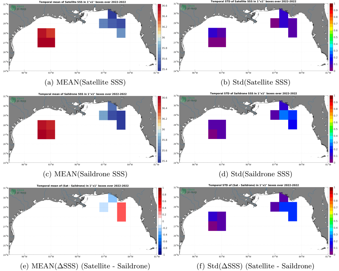
Figure 6: Temporal mean (left) and Std (right) of SSS from SMAP SSS L3 v5 - Monthly (RSS) (top), Saildrone (middle), and of \Delta\text{SSS}(\text{Satellite} - \text{Saildrone}) . Only match-up pairs are used to generate these maps.
