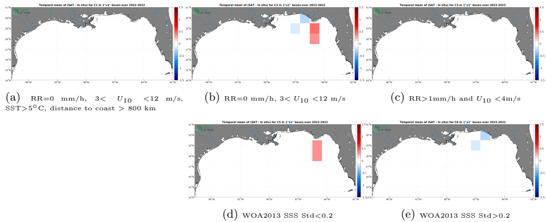
Figure 12: Temporal mean gridded over spatial boxes of size 1^{\circ}\times 1^{\circ} of \Delta\text{SSS} (SMAP SSS L3 v5 - Monthly (RSS) - Saildrone) for 5 different subdatasets corresponding to:RR=0 mm/h, 3 < U_{10} < 12 m/s, SST >5^{\circ}\text{C} , distance to coast > 800 km (a), RR=0 mm/h, 3 < U_{10} < 12 m/s (b), RR >1 mm/h and U_{10} < 4 m/s (c), WOA2013 SSS Std <0.2 (d), WOA2013 SSS Std >0.2 (e).
