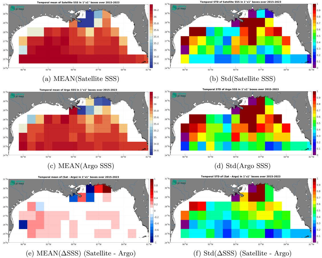
Figure 6: Temporal mean (left) and Std (right) of SSS from SMAP SSS L3 v5 - Monthly (RSS) (top), Argo (middle), and of \Delta\text{SSS} (Satellite - Argo). Only match-up pairs are used to generate these maps.
