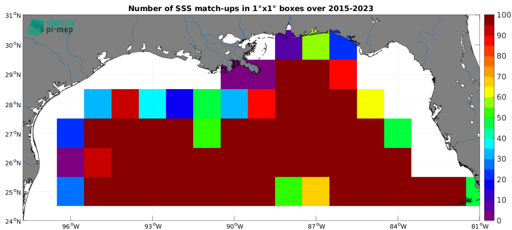
Figure 4: Number of SSS match-ups between Argo SSS and the SMAP SSS L3 v5 - Monthly (RSS) SSS product for the Mississippi river plume Pi-MEP region over 1^\circ \times 1^\circ boxes and for the full satellite product period.
