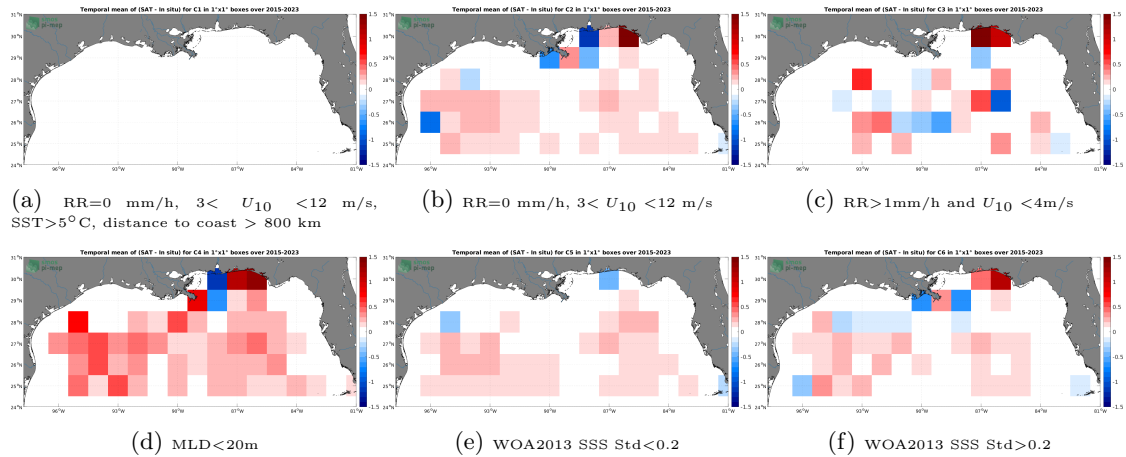
Figure 12: Temporal mean gridded over spatial boxes of size 1^{\circ}\times 1^{\circ} of \Delta\text{SSS} (SMAP SSS L3 v5 - Monthly (RSS) - Argo) for 6 different subdatasets corresponding to: \text{RR}=0 mm/h, 3 < U_{10} < 12 m/s, \text{SST} > 5^{\circ}\text{C} , distance to coast > 800 km (a), \text{RR}=0 mm/h, 3 < U_{10} < 12 m/s (b), \text{RR} > 1\text{mm/h} and U_{10} < 4\text{m/s} (c), \text{MLD} < 20\text{m} (d), WOA2013 SSS Std < 0.2 (e), WOA2013 SSS Std > 0.2 (f).
