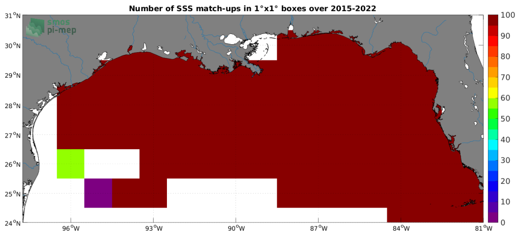
Figure 4: Number of SSS match-ups between TSG (SAMOS) SSS and the SMAP SSS L3 v4 - 8-Day running (RSS) SSS product for the Mississippi river plume Pi-MEP region over 1^\circ \times 1^\circ boxes and for the full satellite product period.
