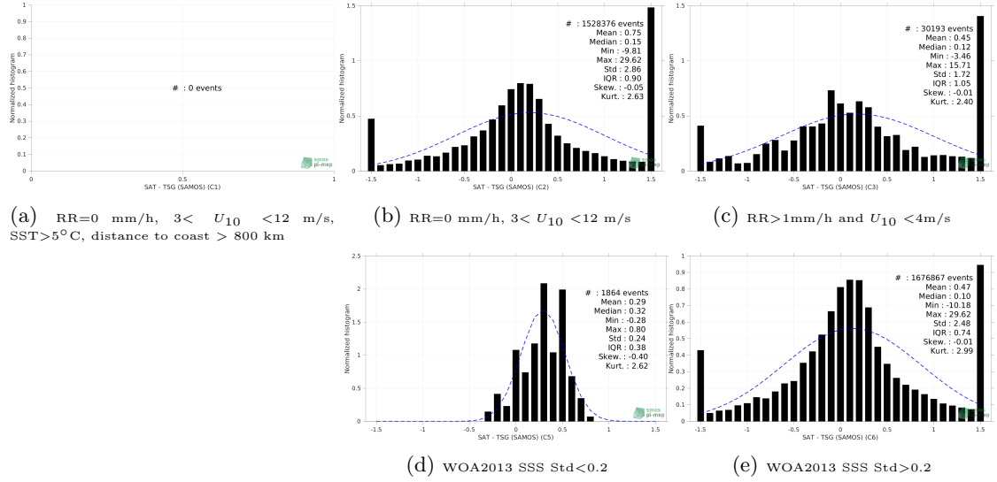
Figure 13: Normalized histogram of \Delta SSS (SMAP SSS L3 v4 - 8-Day running (RSS) - TSG (SAMOS)) for 5 different subdatasets corresponding to: RR=0 mm/h, 3 < U_{10} < 12 m/s, SST > 5°C, distance to coast > 800 km (a), RR=0 mm/h, 3 < U_{10} < 12 m/s (b), RR > 1mm/h and U_{10} < 4 m/s (c), WOA2013 SSS Std < 0.2 (d), WOA2013 SSS Std > 0.2 (e).
