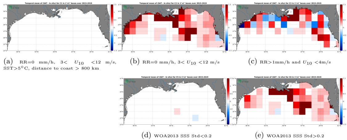
Figure 12: Temporal mean gridded over spatial boxes of size 1^{\circ}\times 1^{\circ} of \Delta\text{SSS} (SMAP-L3-RSS-V4-8DAY-RUNNING - TSG-SAMOS) for 5 different subdatasets corresponding to:RR=0 mm/h, 3 < U_{10} < 12 m/s, SST >5^{\circ}\text{C} , distance to coast > 800 km (a), RR=0 mm/h, 3 < U_{10} < 12 m/s (b), RR >1 mm/h and U_{10} < 4 m/s (c), WOA2013 SSS Std <0.2 (d), WOA2013 SSS Std >0.2 (e).
