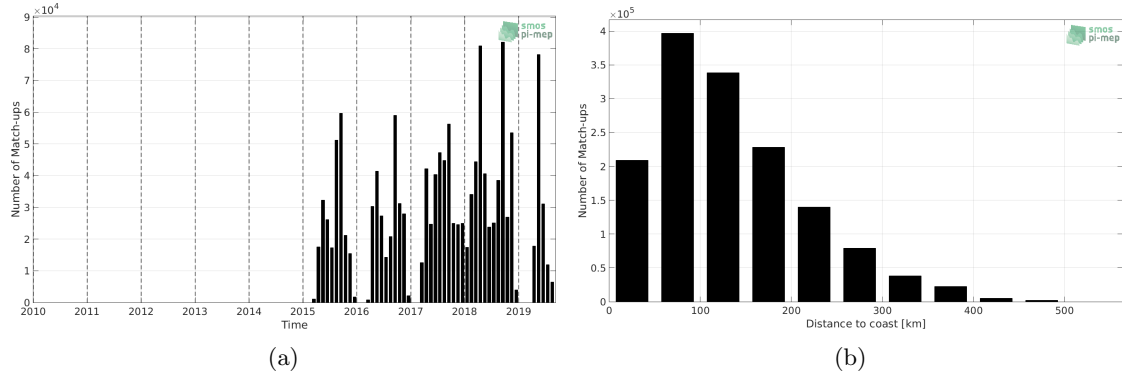
Figure 1: Number of match-ups between TSG-SAMOS and SMAP-L3-RSS-V4-8DAY-RUNNING SSS as a function of time (a) and as function of the distance to coast (b) over the Mississippi river plume Pi-MEP region and for the full satellite product period.
