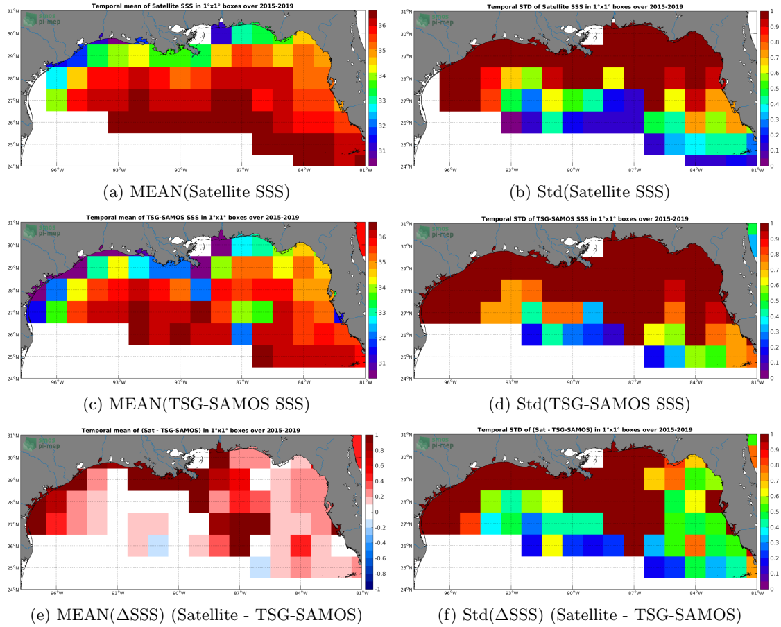
Figure 6: Temporal mean (left) and Std (right) of SSS from SMAP-L3-RSS-V4-8DAY-RUNNING (top), TSG-SAMOS (middle), and of \Delta SSS (Satellite - TSG-SAMOS). Only match-up pairs are used to generate these maps.
