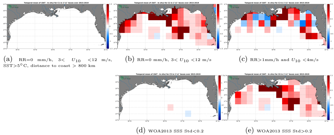
Figure 12: Temporal mean gridded over spatial boxes of size 1^\circ \times 1^\circ of \Delta SSS (SMAP-L3-RSS-V4-8DAY-RUNNING - TSG-SAMOS) for 5 different subdatasets corresponding to:RR=0 mm/h, 3 < U_{10} < 12 m/s, SST >5^\circ\text{C} , distance to coast > 800 km (a), RR=0 mm/h, 3 < U_{10} < 12 m/s (b), RR >1 mm/h and U_{10} < 4 m/s (c), WOA2013 SSS Std <0.2 (d), WOA2013 SSS Std >0.2 (e).
