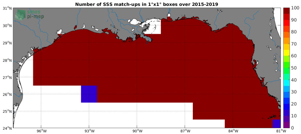
Figure 4: Number of SSS match-ups between TSG-SAMOS SSS and the SMAP-L3-RSS-V4-8DAY-RUNNING SSS product for the Mississippi river plume Pi-MEP region over 1^\circ \times 1^\circ boxes and for the full satellite product period.
