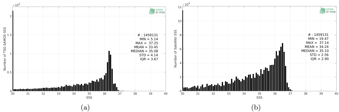
Figure 2: Histograms of SSS from TSG-SAMOS (a) and SMAP-L3-RSS-V4-8DAY-RUNNING (b) considering all match-up pairs per bins of 0.1 over the Mississippi river plume Pi-MEP region and for the full satellite product period.
