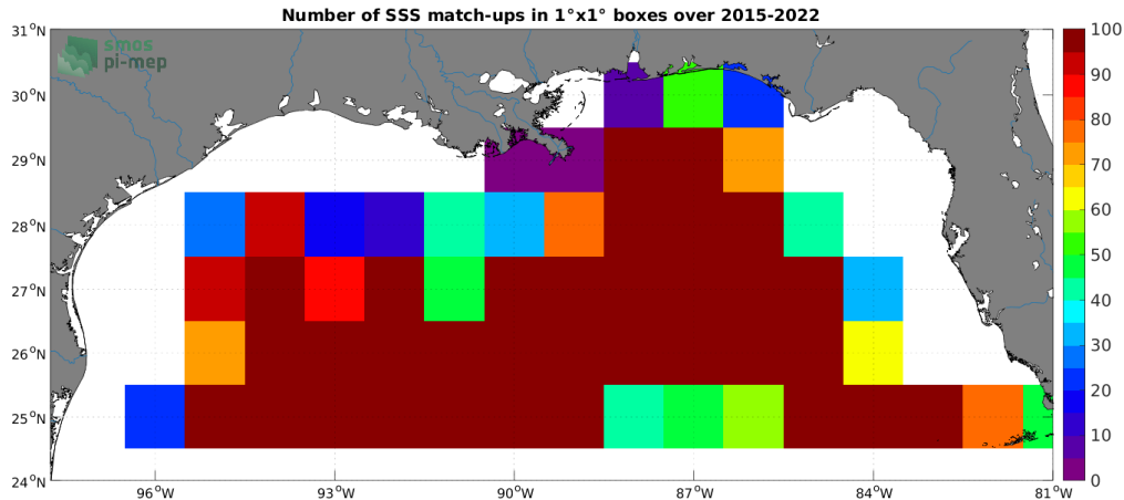
Figure 4: Number of SSS match-ups between Argo SSS and the SMAP SSS L3 v4 - 8-Day running (RSS) SSS product for the Mississippi river plume Pi-MEP region over 1^{\circ} \times 1^{\circ} boxes and for the full satellite product period.
