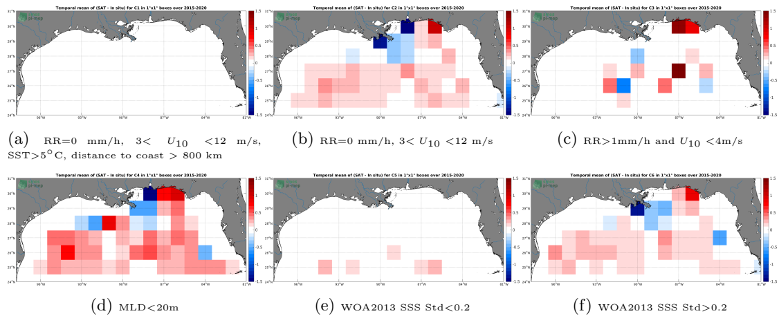
Figure 12: Temporal mean gridded over spatial boxes of size 1^{\circ}\times 1^{\circ} of \Delta\text{SSS} (SMAP-L3-RSS-V4-8DAY-RUNNING - Argo) for 6 different subdatasets corresponding to:RR=0 mm/h, 3 < U_{10} < 12 m/s, SST > 5^{\circ}\text{C} , distance to coast > 800 km (a), RR=0 mm/h, 3 < U_{10} < 12 m/s (b), RR > 1 mm/h and U_{10} < 4 m/s (c),MLD < 20\text{m} (d),WOA2013 SSS Std < 0.2 (e),WOA2013 SSS Std > 0.2 (f).
