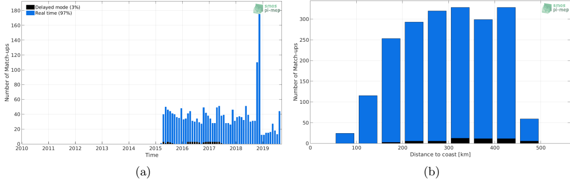
Figure 1: Number of match-ups between Argo and SMAP-L3-RSS-V4-8DAY-RUNNING SSS as a function of time (a) and as function of the distance to coast (b) over the Mississippi river plume Pi-MEP region and for the full satellite product period.
