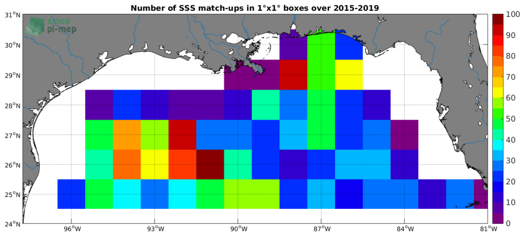
Figure 4: Number of SSS match-ups between Argo SSS and the SMAP-L3-RSS-V4-8DAY-RUNNING SSS product for the Mississippi river plume Pi-MEP region over 1°x1° boxes and for the full satellite product period.
