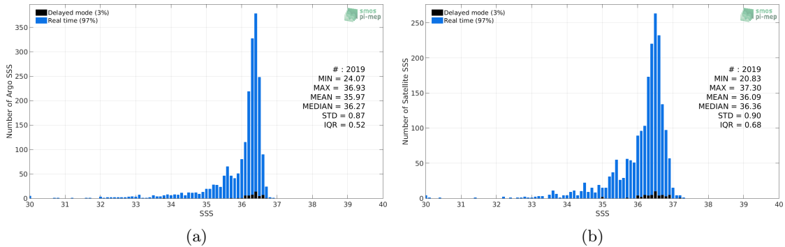
Figure 2: Histograms of SSS from Argo (a) and SMAP-L3-RSS-V4-8DAY-RUNNING (b) considering all match-up pairs per bins of 0.1 over the Mississippi river plume Pi-MEP region and for the full satellite product period.
