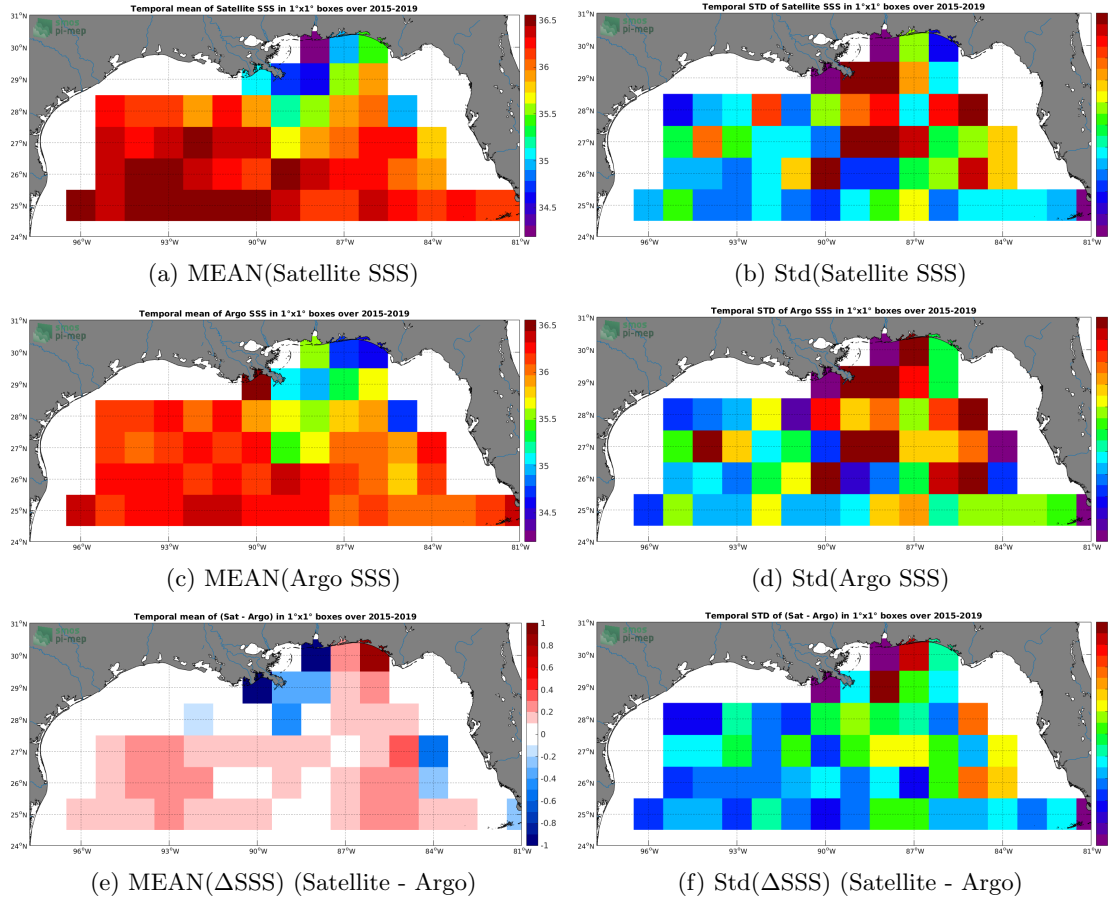
Figure 6: Temporal mean (left) and Std (right) of SSS from SMAP-L3-RSS-V4-8DAY-RUNNING (top), Argo (middle), and of \Delta SSS (Satellite - Argo). Only match-up pairs are used to generate these maps.
