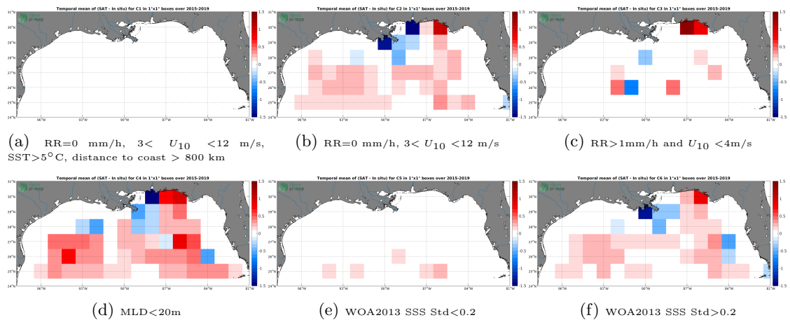
Figure 12: Temporal mean gridded over spatial boxes of size 1^\circ \times 1^\circ of \Delta SSS (SMAP-L3-RSS-V4-8DAY-RUNNING - Argo) for 6 different subdatasets corresponding to:RR=0 mm/h, 3 < U_{10} < 12 m/s, SST >5^\circ C, distance to coast > 800 km (a), RR=0 mm/h, 3 < U_{10} < 12 m/s (b), RR >1 mm/h and U_{10} < 4 m/s (c),MLD <20 m (d),WOA2013 SSS Std <0.2 (e),WOA2013 SSS Std >0.2 (f).
