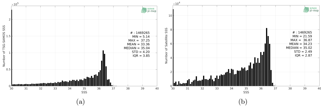
Figure 2: Histograms of SSS from TSG-SAMOS (a) and SMAP-L3-RSS-V4-MONTHLY (b) considering all match-up pairs per bins of 0.1 over the Mississippi river plume Pi-MEP region and for the full satellite product period.
