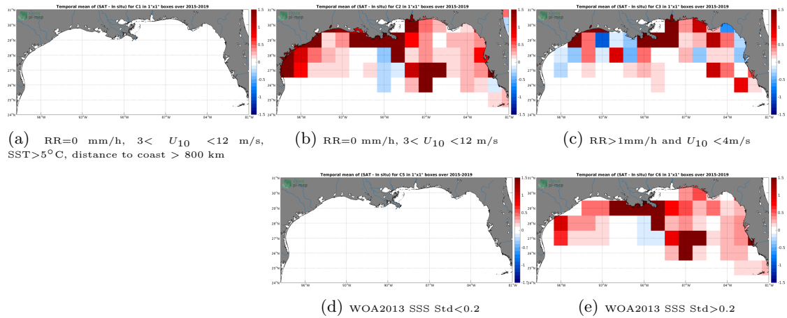
Figure 12: Temporal mean gridded over spatial boxes of size 1^\circ \times 1^\circ of \Delta SSS (SMAP-L3-RSS-V4-MONTHLY - TSG-SAMOS) for 5 different subdatasets corresponding to:RR=0 mm/h, 3 < U_{10} < 12 m/s, SST > 5^\circ\text{C} , distance to coast > 800 km (a), RR=0 mm/h, 3 < U_{10} < 12 m/s (b), RR > 1 mm/h and U_{10} < 4 m/s (c), WOA2013 SSS Std < 0.2 (d), WOA2013 SSS Std > 0.2 (e).
