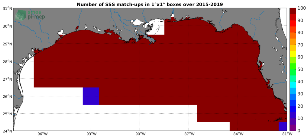
Figure 4: Number of SSS match-ups between TSG-SAMOS SSS and the SMAP-L3-RSS-V4-MONTHLY SSS product for the Mississippi river plume Pi-MEP region over 1^\circ \times 1^\circ boxes and for the full satellite product period.
