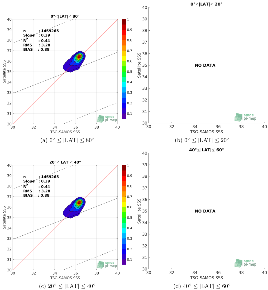
Figure 9: Contour maps of the concentration of SMAP-L3-RSS-V4-MONTHLY SSS (y-axis) versus TSG-SAMOS SSS (x-axis) at match-up pairs for different latitude bands. For each plot, the red line shows x=y . The black thin and dashed lines indicate a linear fit through the data cloud and the \pm 95\% confidence levels, respectively. The number match-up pairs n , the slope and R^2 coefficient of the linear fit, the root mean square (RMS) and the mean bias between satellite and in situ data are indicated for each latitude band in each plots.
