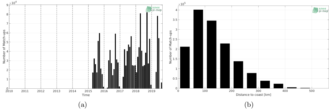
Figure 1: Number of match-ups between TSG-SAMOS and SMAP-L3-RSS-V4-MONTHLY SSS as a function of time (a) and as function of the distance to coast (b) over the Mississippi river plume Pi-MEP region and for the full satellite product period.
