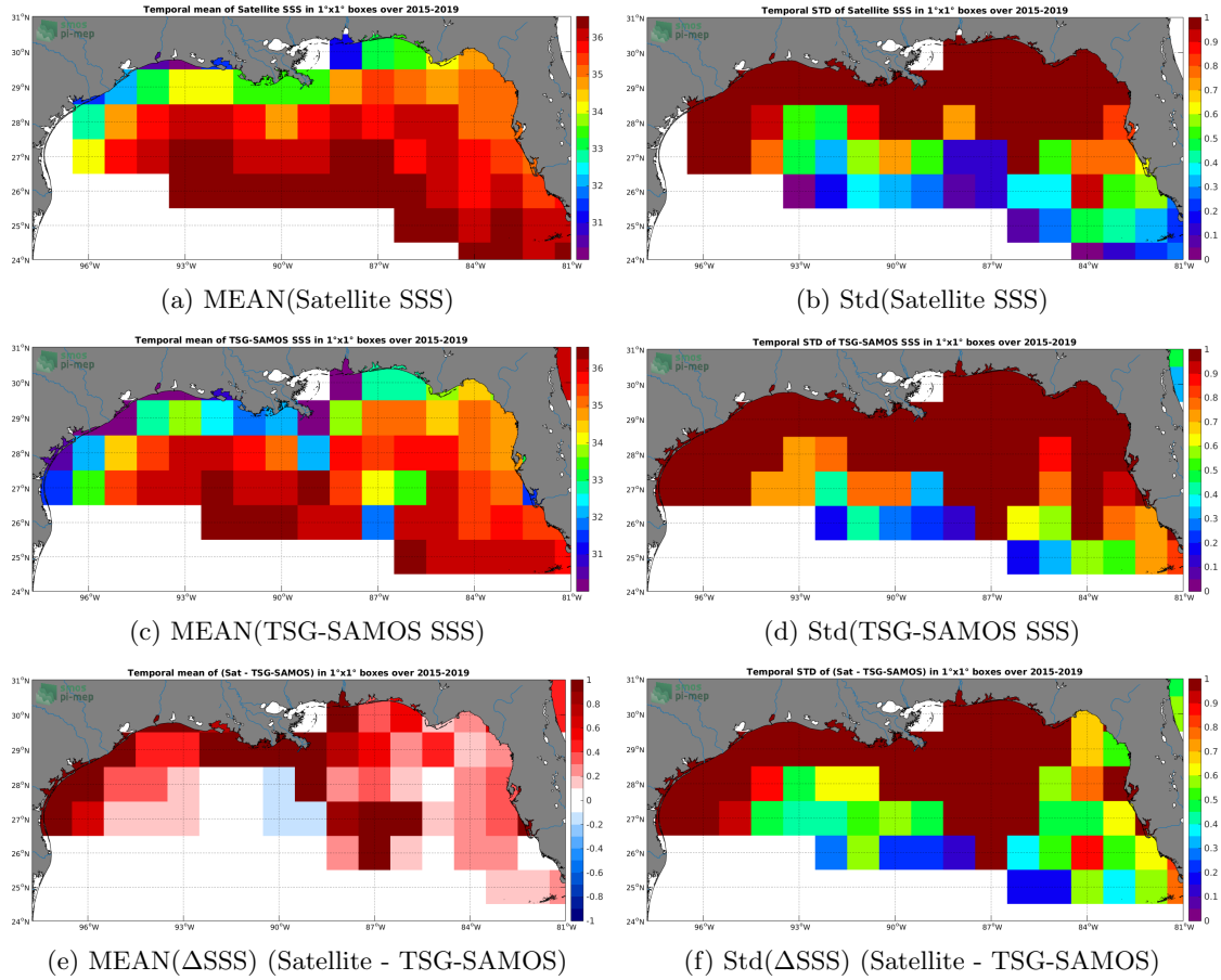
Figure 6: Temporal mean (left) and Std (right) of SSS from SMAP-L3-RSS-V4-MONTHLY (top), TSG-SAMOS (middle), and of \Delta SSS (Satellite - TSG-SAMOS). Only match-up pairs are used to generate these maps.
