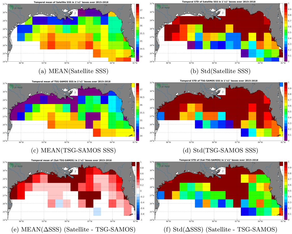
Figure 6: Temporal mean (left) and Std (right) of SSS from SMAP-L3-RSS-V3-8DAY-RUNNING-40KM (top), TSG-SAMOS (middle), and of \Delta SSS (Satellite - TSG-SAMOS). Only match-up pairs are used to generate these maps.
