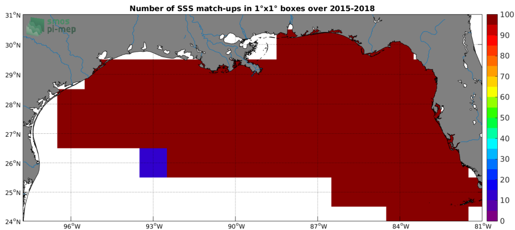
Figure 4: Number of SSS match-ups between TSG-SAMOS SSS and the SMAP-L3-RSS-V3-8DAY-RUNNING-40KM SSS product for the Mississippi river plume Pi-MEP region over 1^\circ \times 1^\circ boxes and for the full satellite product period.
