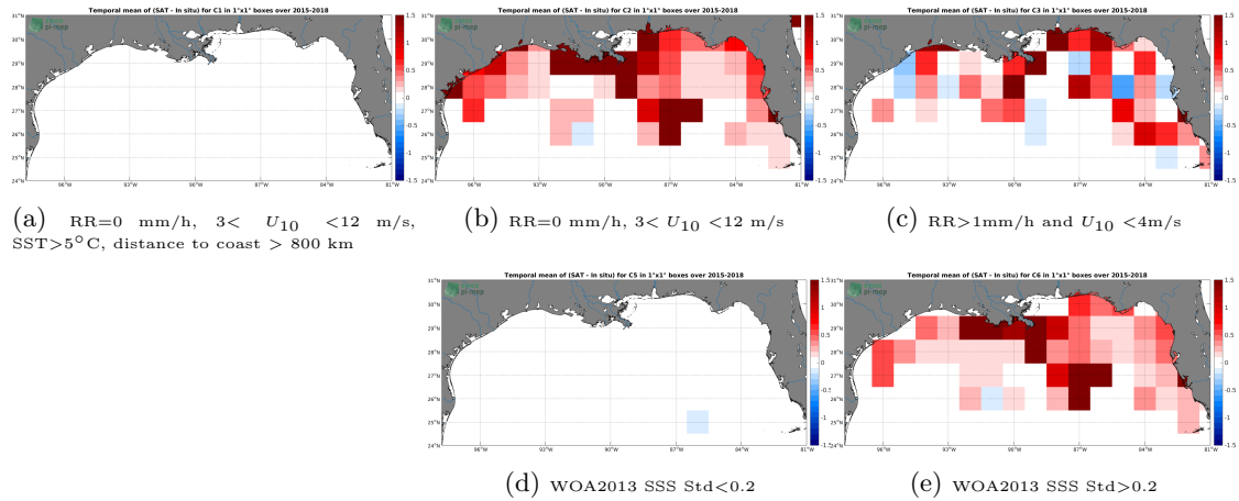
Figure 12: Temporal mean gridded over spatial boxes of size 1^\circ \times 1^\circ of \Delta SSS (SMAP-L3-RSS-V3-8DAY-RUNNING-40KM - TSG-SAMOS) for 5 different subdatasets corresponding to:RR=0 mm/h, 3 < U_{10} < 12 m/s, SST >5^\circ C, distance to coast > 800 km (a), RR=0 mm/h, 3 < U_{10} < 12 m/s (b), RR >1 mm/h and U_{10} < 4 m/s (c), WOA2013 SSS Std <0.2 (d), WOA2013 SSS Std >0.2 (e).
