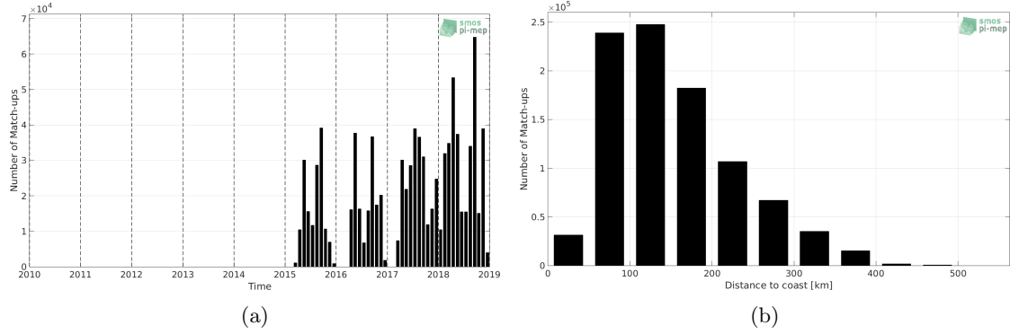
Figure 1: Number of match-ups between TSG-SAMOS and SMAP-L3-RSS-V3-8DAY-RUNNING-40KM SSS as a function of time (a) and as function of the distance to coast (b) over the Mississippi river plume Pi-MEP region and for the full satellite product period.
