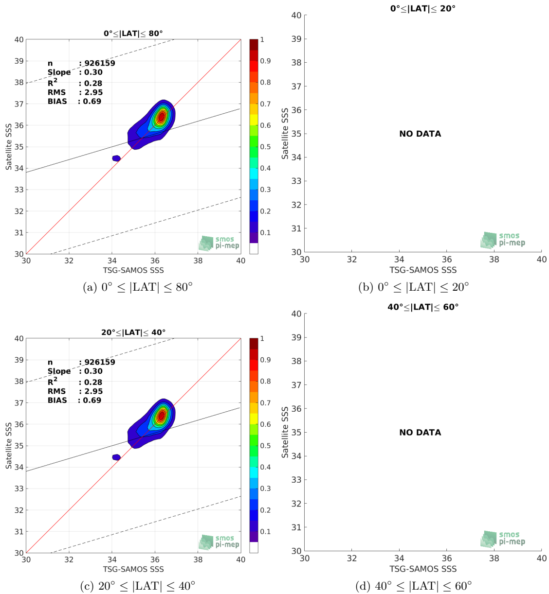
Figure 9: Contour maps of the concentration of SMAP-L3-RSS-V3-8DAY-RUNNING-40KM SSS (y-axis) versus TSG-SAMOS SSS (x-axis) at match-up pairs for different latitude bands. For each plot, the red line shows x=y . The black thin and dashed lines indicate a linear fit through the data cloud and the \pm 95\% confidence levels, respectively. The number match-up pairs n , the slope and R^2 coefficient of the linear fit, the root mean square (RMS) and the mean bias between satellite and in situ data are indicated for each latitude band in each plots.
