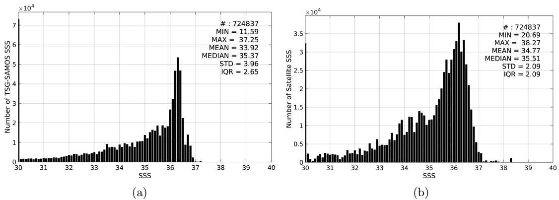
Figure 2: Histograms of SSS from TSG-SAMOS (a) and SMAP-L3-RSS-V2-8DAY-RUNNING-40KM (b) considering all match-up pairs per bins of 0.1 over the Mississippi river plume Pi-MEP region and for the full satellite product period.
