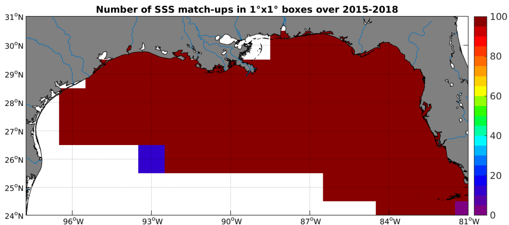
Figure 4: Number of SSS match-ups between TSG-SAMOS SSS and the SMAP-L3-RSS-V2-8DAY-RUNNING-40KM SSS product for the Mississippi river plume Pi-MEP region over 1^\circ \times 1^\circ boxes and for the full satellite product period.
