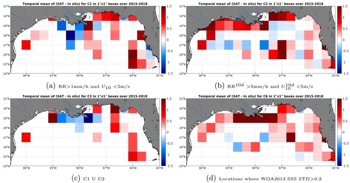
Figure 12: Temporal mean gridded over spatial boxes of size 1^\circ \times 1^\circ of \Delta SSS (SMAP-L3-RSS-V2-8DAY-RUNNING-40KM - TSG-SAMOS) for 4 different subdatasets corresponding to:RR > 1 mm/h and U_{10} < 5 m/s (a), RR^{10d} > 5 mm/h and U_{10}^{10d} < 5 m/s (b), C1 U C2 (c),Locations where WOA2013 SSS STD > 0.2 (d).
