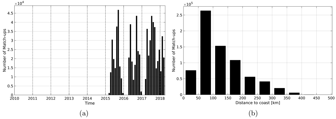
Figure 1: Number of match-ups between TSG-SAMOS and SMAP-L3-RSS-V2-8DAY-RUNNING-40KM SSS as a function of time (a) and as function of the distance to coast (b) over the Mississippi river plume Pi-MEP region and for the full satellite product period.
