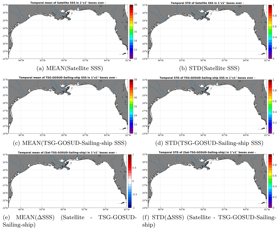
Figure 6: Temporal mean (left) and STD (right) of SSS from SMAP-L3-RSS-V2-8DAY-RUNNING-40KM (top), TSG-GOSUD-Sailing-ship (middle), and of \Delta SSS (Satellite - TSG-GOSUD-Sailing-ship). Only match-up pairs are used to generate these maps.
