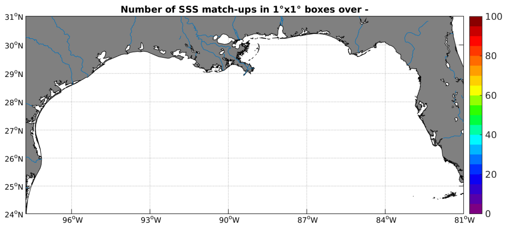
Figure 4: Number of SSS match-ups between TSG-GOSUD-Research-vessel SSS and the SMAP-L3-RSS-V2-8DAY-RUNNING-40KM SSS product for the Mississippi river plume Pi-MEP region over 1^{\circ} \times 1^{\circ} boxes and for the full satellite product period.
