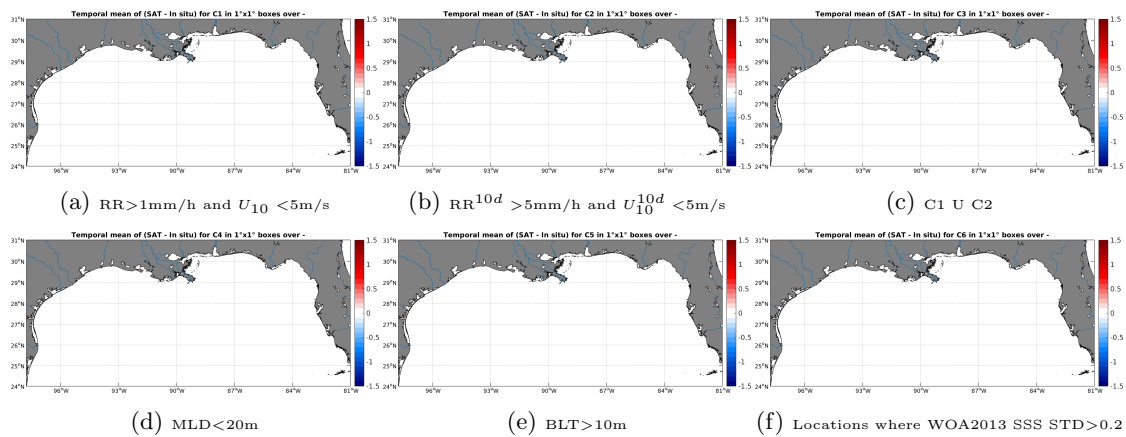
Figure 12: Temporal mean gridded over spatial boxes of size 1^\circ \times 1^\circ of \Delta SSS (SMAP-L3-RSS-V2-8DAY-RUNNING-40KM - Sea mammals) for 6 different subdatasets corresponding to:RR >1 mm/h and U_{10} < 5 m/s (a), RR ^{10d} > 5 mm/h and U_{10}^{10d} < 5 m/s (b), C1 U C2 (c),MLD <20 m (d),BLT >10 m (e),Locations where WOA2013 SSS STD >0.2 (f).
