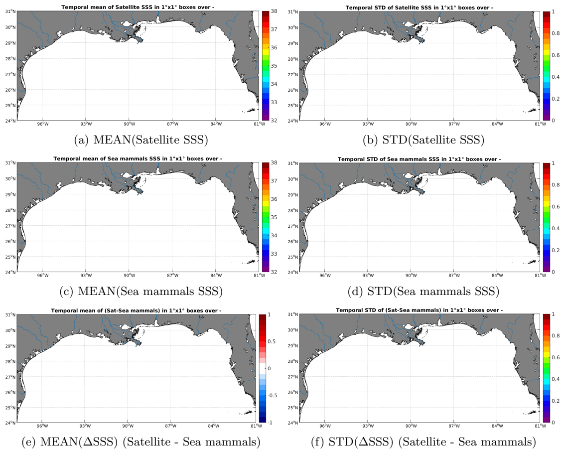
Figure 6: Temporal mean (left) and STD (right) of SSS from SMAP-L3-RSS-V2-8DAY-RUNNING-40KM (top), Sea mammals (middle), and of \Delta SSS (Satellite - Sea mammals). Only match-up pairs are used to generate these maps.
