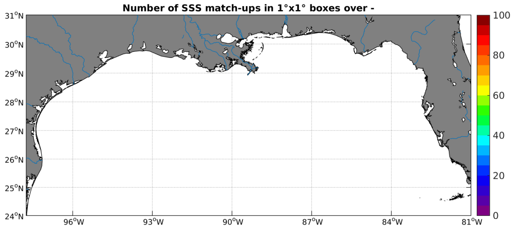
Figure 3: Number of SSS match-ups between Surface drifters SSS and the SMAP-L3-RSS-V2-8DAY-RUNNING-40KM SSS product for the Mississippi river plume Pi-MEP region over 1^\circ \times 1^\circ boxes and for the full satellite product period.
