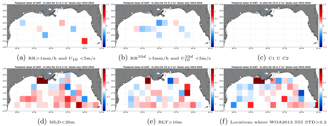
Figure 12: Temporal mean gridded over spatial boxes of size 1°x1° of \Delta SSS (SMAP-L3-RSS-V2-8DAY-RUNNING-40KM - Argo) for 6 different subdatasets corresponding to:RR>1mm/h and U_{10} < 5 m/s (a), RR^{10d} > 5 mm/h and U_{10}^{10d} < 5 m/s (b), C1 U C2 (c),MLD<20m (d),BLT>10m (e),Locations where WOA2013 SSS STD>0.2 (f).
