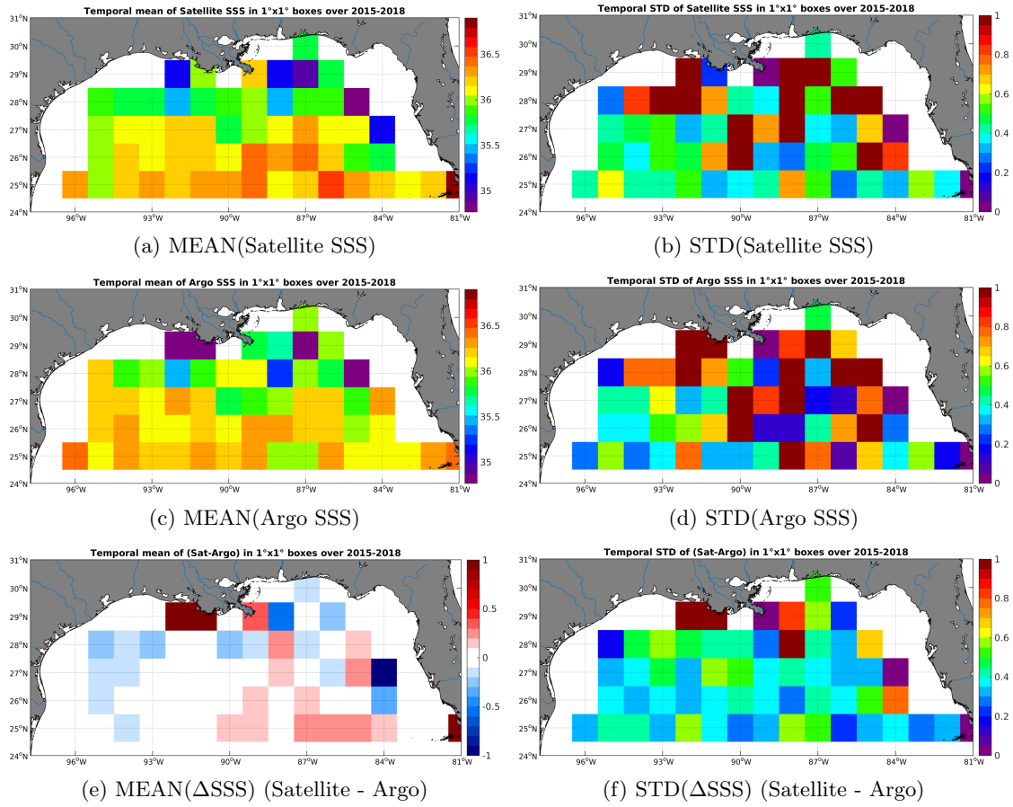
Figure 6: Temporal mean (left) and STD (right) of SSS from SMAP-L3-RSS-V2-8DAY-RUNNING-40KM (top), Argo (middle), and of \Delta SSS (Satellite - Argo). Only match-up pairs are used to generate these maps.
