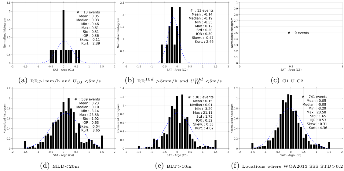
Figure 13: Normalized histogram of \Delta SSS (SMAP-L3-RSS-V2-8DAY-RUNNING-40KM - Argo) for 6 different subdatasets corresponding to: RR > 1mm/h and U_{10} < 5 m/s (a), RR^{10d} > 5 mm/h and U_{10}^{10d} < 5 m/s (b), C1 U C2 (c), MLD < 20m (d), BLT > 10m (e), Locations where WOA2013 SSS STD > 0.2 (f).
