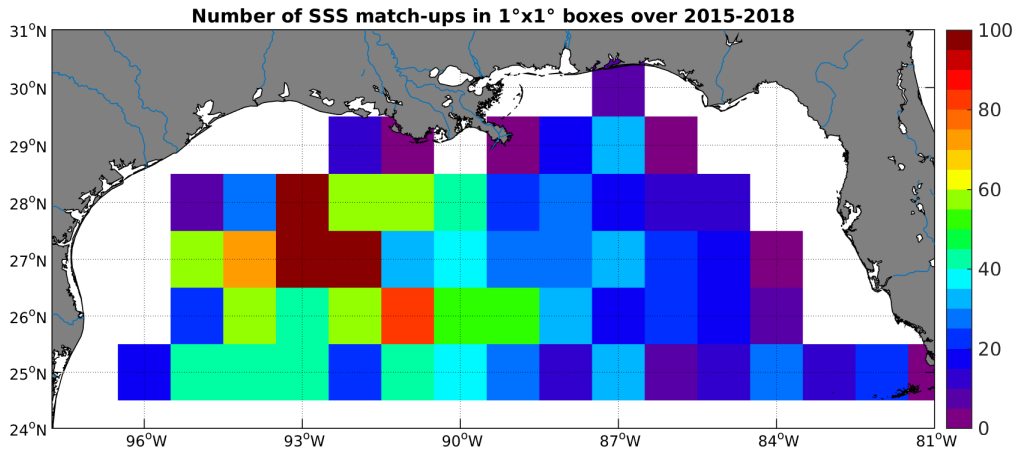
Figure 4: Number of SSS match-ups between Argo SSS and the SMAP-L3-RSS-V2-8DAY-RUNNING-40KM SSS product for the Mississippi river plume Pi-MEP region over 1^\circ \times 1^\circ boxes and for the full satellite product period.
