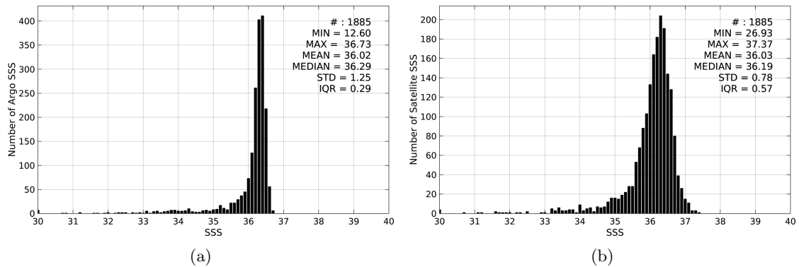
Figure 2: Histograms of SSS from Argo (a) and SMAP-L3-RSS-V2-8DAY-RUNNING-40KM (b) considering all match-up pairs per bins of 0.1 over the Mississippi river plume Pi-MEP region and for the full satellite product period.
