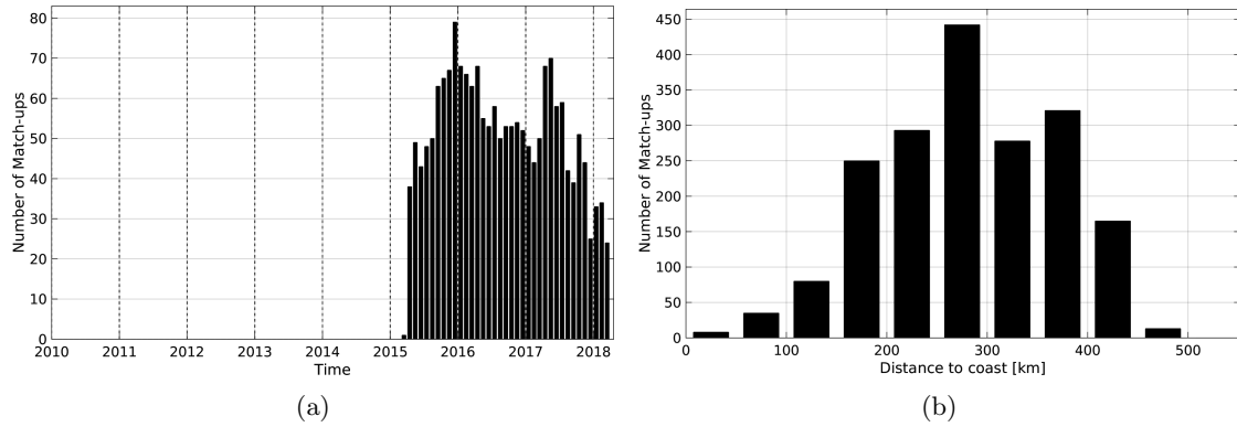
Figure 1: Number of match-ups between Argo and SMAP-L3-RSS-V2-8DAY-RUNNING-40KM SSS as a function of time (a) and as function of the distance to coast (b) over the Mississippi river plume Pi-MEP region and for the full satellite product period.
