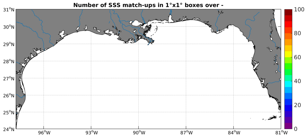
Figure 4: Number of SSS match-ups between TSG-GOSUD-Sailing-ship SSS and the SMAP-L3-RSS-V2-8DAY-RUNNING-70KM SSS product for the Mississippi river plume Pi-MEP region over 1^\circ \times 1^\circ boxes and for the full satellite product period.
