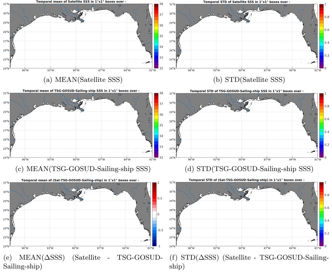
Figure 6: Temporal mean (left) and STD (right) of SSS from SMAP-L3-RSS-V2-8DAY-RUNNING-70KM (top), TSG-GOSUD-Sailing-ship (middle), and of \Delta SSS (Satellite - TSG-GOSUD-Sailing-ship). Only match-up pairs are used to generate these maps.
