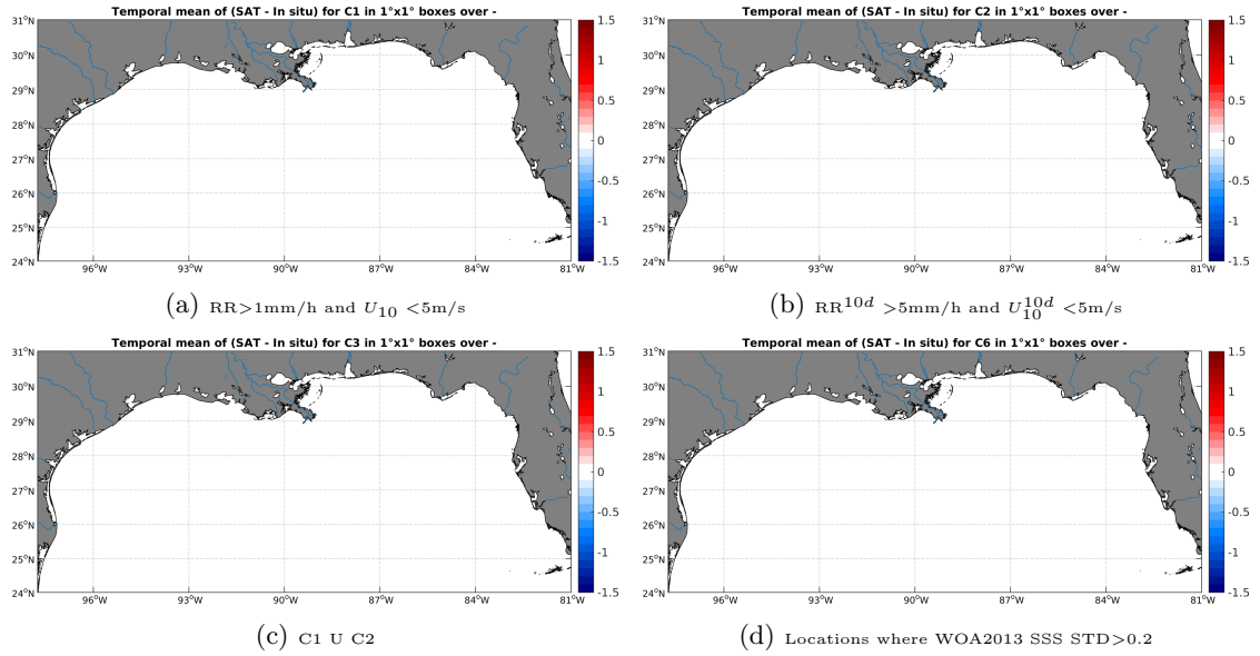
Figure 12: Temporal mean gridded over spatial boxes of size 1^\circ \times 1^\circ of \Delta SSS (SMAP-L3-RSS-V2-8DAY-RUNNING-70KM - TSG-GOSUD-Sailing-ship) for 4 different subdatasets corresponding to: RR > 1\text{mm/h} and U_{10} < 5\text{m/s} (a), RR^{10d} > 5\text{mm/h} and U_{10}^{10d} < 5\text{m/s} (b), C1 U C2 (c), Locations where WOA2013 SSS STD > 0.2 (d).
