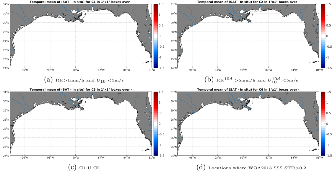
Figure 12: Temporal mean gridded over spatial boxes of size 1^\circ \times 1^\circ of \Delta SSS (SMAP-L3-RSS-V2-8DAY-RUNNING-70KM - TSG-GOSUD-Research-vessel) for 4 different subdatasets corresponding to: RR > 1\text{mm/h} and U_{10} < 5\text{m/s} (a), RR^{10d} > 5\text{mm/h} and U_{10}^{10d} < 5\text{m/s} (b), C1 U C2 (c), Locations where WOA2013 SSS STD > 0.2 (d).
