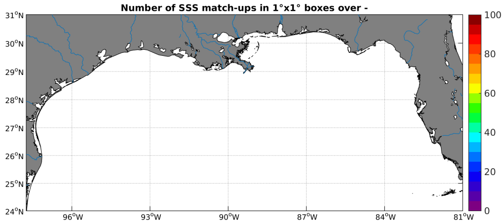
Figure 4: Number of SSS match-ups between TSG-GOSUD-Research-vessel SSS and the SMAP-L3-RSS-V2-8DAY-RUNNING-70KM SSS product for the Mississippi river plume Pi-MEP region over 1^\circ \times 1^\circ boxes and for the full satellite product period.
