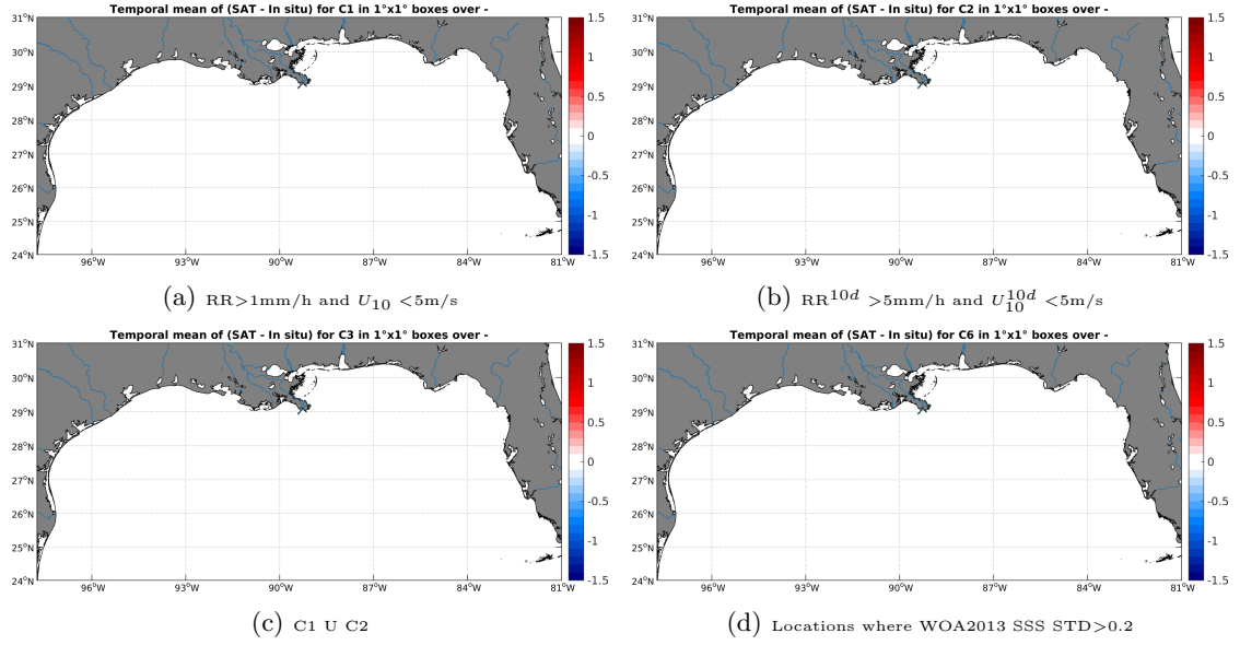
Figure 11: Temporal mean gridded over spatial boxes of size 1^\circ \times 1^\circ of \Delta SSS (SMAP-L3-RSS-V2-8DAY-RUNNING-70KM - Surface drifters) for 4 different subdatasets corresponding to: RR > 1\text{mm/h} and U_{10} < 5\text{m/s} (a), RR^{10d} > 5\text{mm/h} and U_{10}^{10d} < 5\text{m/s} (b), C1 U C2 (c), Locations where WOA2013 SSS STD > 0.2 (d).
