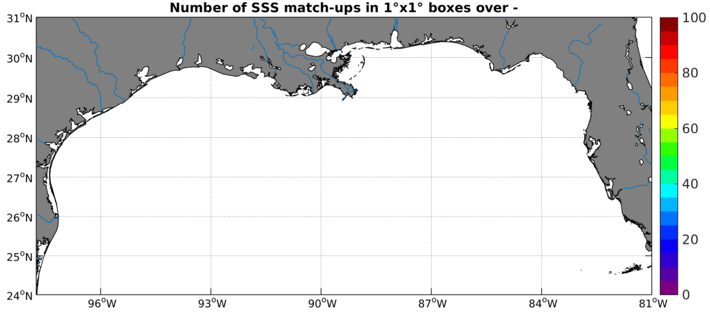
Figure 3: Number of SSS match-ups between Surface drifters SSS and the SMAP-L3-RSS-V2-8DAY-RUNNING-70KM SSS product for the Mississippi river plume Pi-MEP region over 1^\circ \times 1^\circ boxes and for the full satellite product period.
