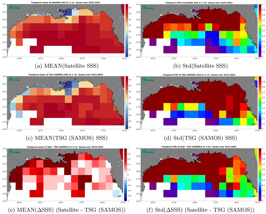
Figure 6: Temporal mean (left) and Std (right) of SSS from SMAP SSS L3 v5.0 - Monthly (JPL) (top), TSG (SAMOS) (middle), and of \Delta SSS (Satellite - TSG (SAMOS)). Only match-up pairs are used to generate these maps.
