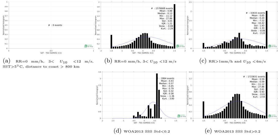
Figure 13: Normalized histogram of \Delta\text{SSS} (SMAP SSS L3 v5.0 - Monthly (JPL) - TSG (SAMOS)) for 5 different subdatasets corresponding to: RR=0 mm/h, 3 < U_{10} < 12 m/s, SST > 5^{\circ}\text{C} , distance to coast > 800 km (a), RR=0 mm/h, 3 < U_{10} < 12 m/s (b), RR > 1\text{mm/h} and U_{10} < 4\text{m/s} (c), WOA2013 SSS Std < 0.2 (d), WOA2013 SSS Std > 0.2 (e).
