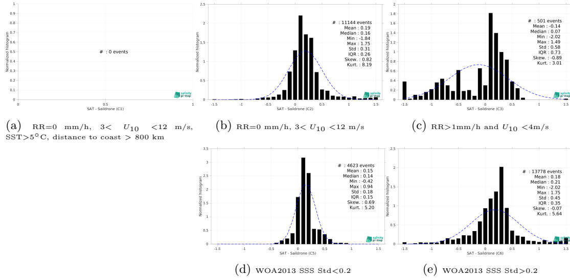
Figure 13: Normalized histogram of \Delta SSS (SMAP SSS L3 v5.0 - Monthly (JPL) - Saldrone) for 5 different subdatasets corresponding to: RR=0 mm/h, 3 < U_{10} < 12 m/s, SST > 5°C, distance to coast > 800 km (a), RR=0 mm/h, 3 < U_{10} < 12 m/s (b), RR > 1mm/h and U_{10} < 4 m/s (c), WOA2013 SSS Std < 0.2 (d), WOA2013 SSS Std > 0.2 (e).
