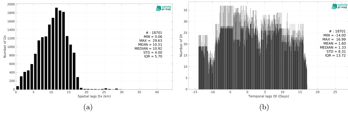
Figure 5: Histograms of the spatial (a) and temporal (b) lags between the location/time of the Saildrone measurement and the date of the corresponding SMAP SSS L3 v5.0 - Monthly (JPL) SSS pixel.
