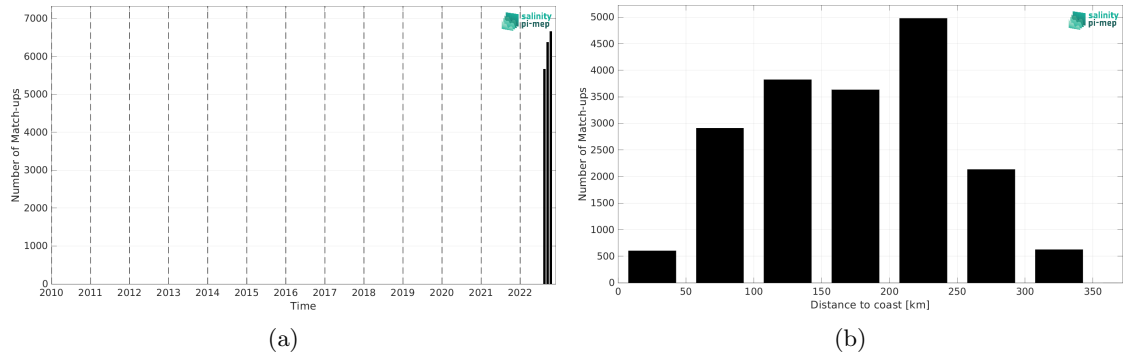
Figure 1: Number of match-ups between Saildrone and SMAP SSS L3 v5.0 - Monthly (JPL) SSS as a function of time (a) and as function of the distance to coast (b) over the Mississippi river plume Pi-MEP region and for the full satellite product period.
