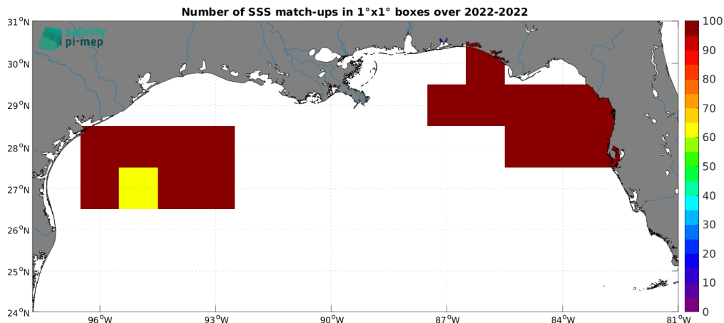
Figure 4: Number of SSS match-ups between Saildrone SSS and the SMAP SSS L3 v5.0 - Monthly (JPL) SSS product for the Mississippi river plume Pi-MEP region over 1^\circ \times 1^\circ boxes and for the full satellite product period.
