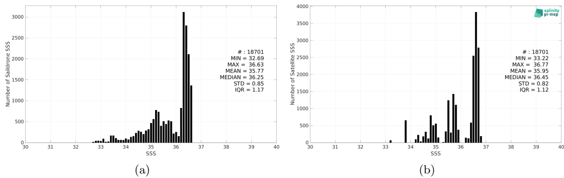
Figure 2: Histograms of SSS from Saildrone (a) and SMAP SSS L3 v5.0 - Monthly (JPL) (b) considering all match-up pairs per bins of 0.1 over the Mississippi river plume Pi-MEP region and for the full satellite product period.
