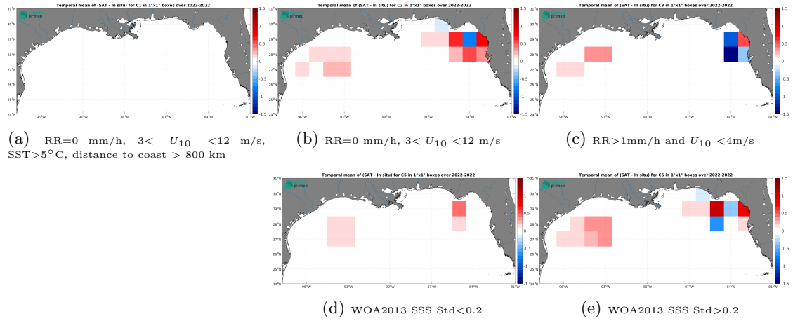
Figure 12: Temporal mean gridded over spatial boxes of size 1^{\circ}\times 1^{\circ} of \Delta\text{SSS} (SMAP SSS L3 v5.0 - Monthly (JPL) - Saildrone) for 5 different subdatasets corresponding to:RR=0 mm/h, 3 < U_{10} < 12 m/s, SST > 5^{\circ}\text{C} , distance to coast > 800 km (a), RR=0 mm/h, 3 < U_{10} < 12 m/s (b), RR > 1 mm/h and U_{10} < 4 m/s (c), WOA2013 SSS Std < 0.2 (d), WOA2013 SSS Std > 0.2 (e).
