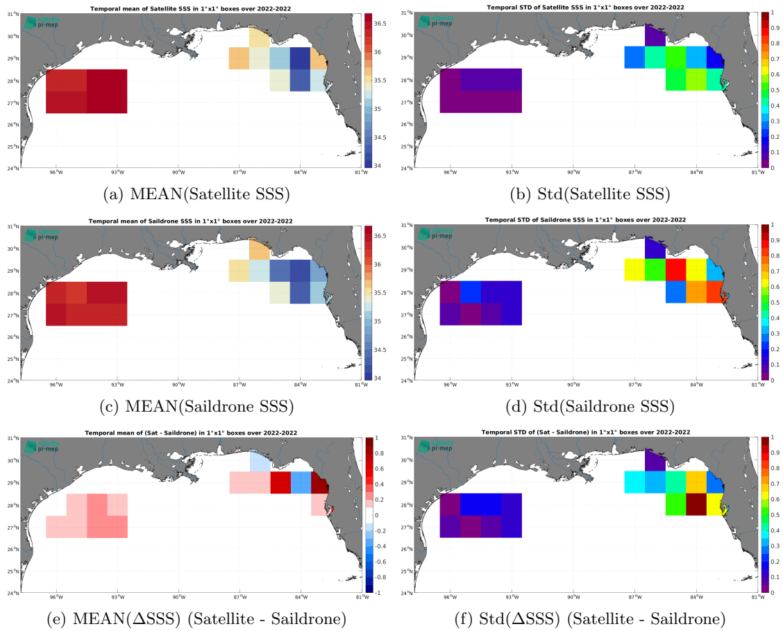
Figure 6: Temporal mean (left) and Std (right) of SSS from SMAP SSS L3 v5.0 - Monthly (JPL) (top), Saildrone (middle), and of \Delta SSS (Satellite - Saildrone). Only match-up pairs are used to generate these maps.
