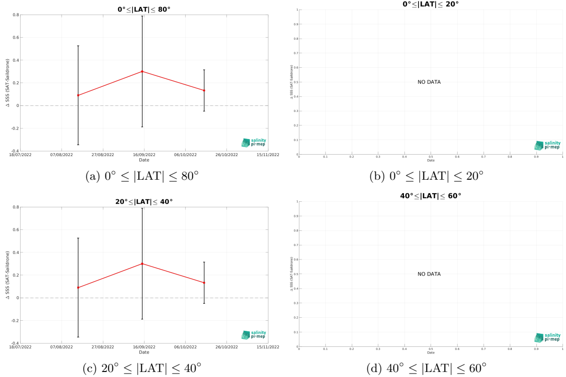
Figure 10: Monthly median (red curves) of \Delta SSS (Satellite - Sairdron) and \pm 1 Std (black vertical thick bars) as function of time for all the collected Pi-MEP match-up pairs estimated over the Mississippi river plume Pi-MEP region and for the full satellite product period are shown for different latitude bands: (a) 80^\circ\text{S}-80^\circ\text{N} , (b) 20^\circ\text{S}-20^\circ\text{N} , (c) 40^\circ\text{S}-20^\circ\text{S} and 20^\circ\text{N}-40^\circ\text{N} and (d) 60^\circ\text{S}-40^\circ\text{S} and 40^\circ\text{N}-60^\circ\text{N} .
