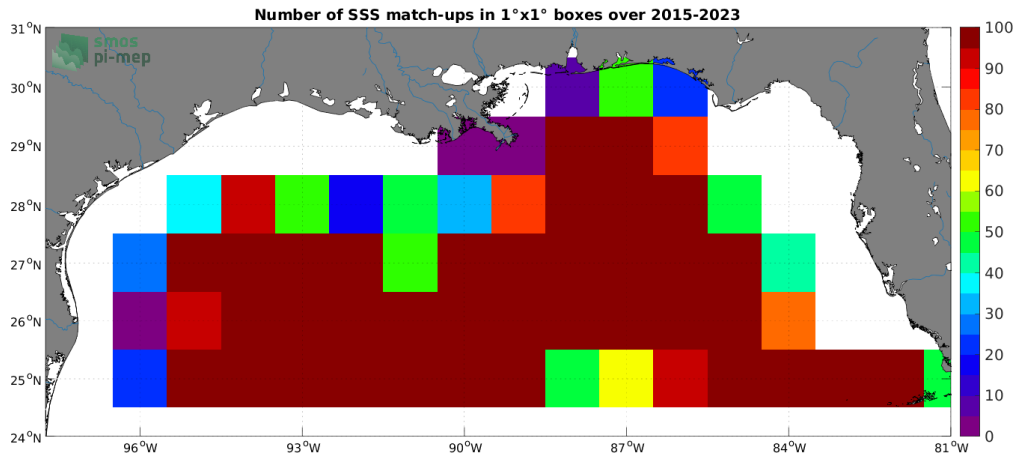
Figure 4: Number of SSS match-ups between Argo SSS and the SMAP SSS L3 v5.0 - Monthly (JPL) SSS product for the Mississippi river plume Pi-MEP region over 1^{\circ} \times 1^{\circ} boxes and for the full satellite product period.
