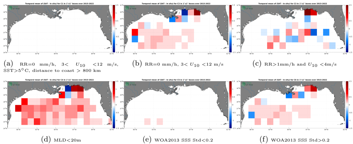
Figure 12: Temporal mean gridded over spatial boxes of size 1^{\circ}\times 1^{\circ} of \Delta\text{SSS} (SMAP SSS L3 v5.0 - Monthly (JPL) - Argo) for 6 different subdatasets corresponding to: \text{RR}=0 mm/h, 3 < U_{10} < 12 m/s, \text{SST} > 5^{\circ}\text{C} , distance to coast > 800 km (a), \text{RR}=0 mm/h, 3 < U_{10} < 12 m/s (b), \text{RR} > 1 mm/h and U_{10} < 4 m/s (c), \text{MLD} < 20\text{m} (d), WOA2013 SSS Std < 0.2 (e), WOA2013 SSS Std > 0.2 (f).
