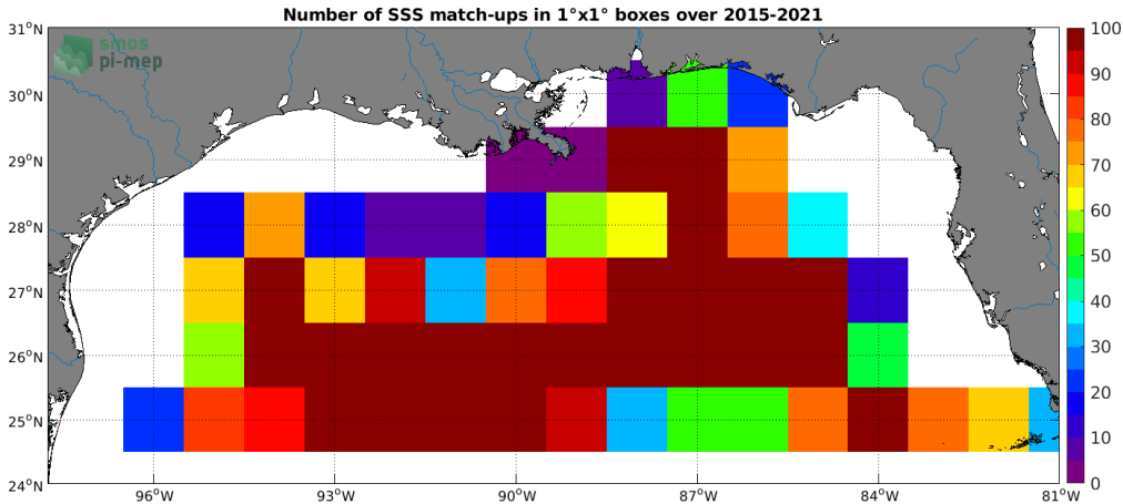
Figure 4: Number of SSS match-ups between Argo SSS and the SMAP SSS L3 v5.0 - Monthly (JPL) SSS product for the Mississippi river plume Pi-MEP region over 1°x1° boxes and for the full satellite product period.
