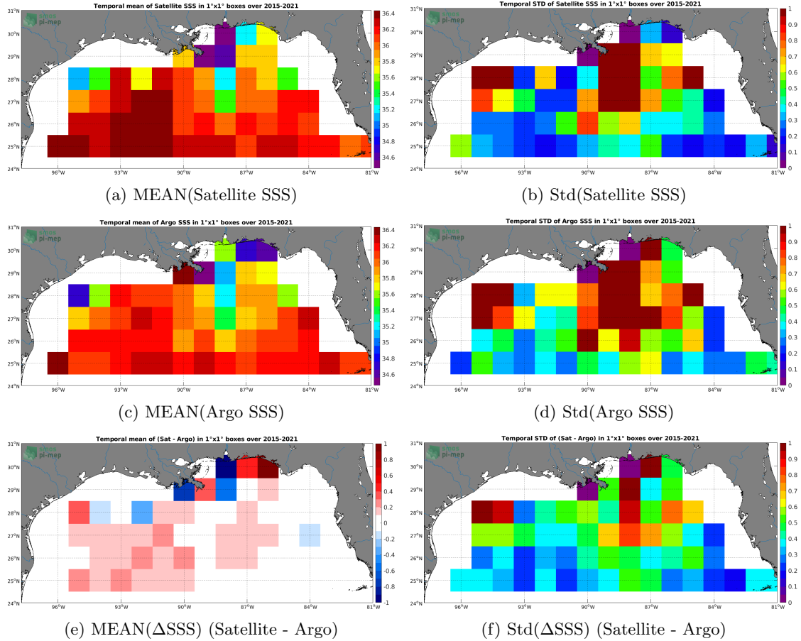
Figure 6: Temporal mean (left) and Std (right) of SSS from SMAP SSS L3 v5.0 - Monthly (JPL) (top), Argo (middle), and of \Delta\text{SSS} (Satellite - Argo). Only match-up pairs are used to generate these maps.
