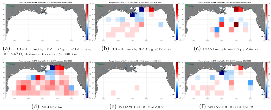
Figure 12: Temporal mean gridded over spatial boxes of size 1^{\circ}\times 1^{\circ} of \Delta\text{SSS} (SMAP-L3-JPL-V4.3-8DAY-RUNNING-60KM - Argo) for 6 different subdatasets corresponding to:RR=0 mm/h, 3 < U_{10} < 12 m/s, SST > 5^{\circ}\text{C} , distance to coast > 800 km (a), RR=0 mm/h, 3 < U_{10} < 12 m/s (b), RR > 1 mm/h and U_{10} < 4 m/s (c),MLD < 20\text{m} (d),WOA2013 SSS Std < 0.2 (e),WOA2013 SSS Std > 0.2 (f).
