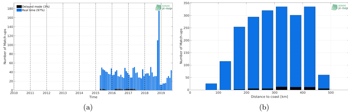
Figure 1: Number of match-ups between Argo and SMAP-L3-JPL-V4.3-8DAY-RUNNING-60KM SSS as a function of time (a) and as function of the distance to coast (b) over the Mississippi river plume Pi-MEP region and for the full satellite product period.
