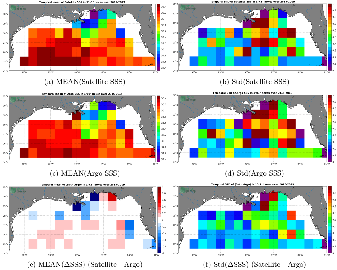
Figure 6: Temporal mean (left) and Std (right) of SSS from SMAP-L3-JPL-V4.3-8DAY-RUNNING-60KM (top), Argo (middle), and of \Delta SSS (Satellite - Argo). Only match-up pairs are used to generate these maps.
