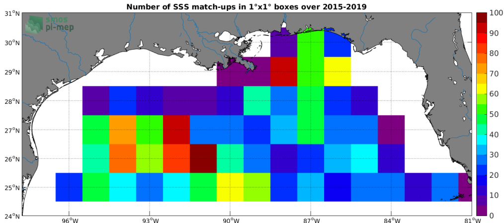
Figure 4: Number of SSS match-ups between Argo SSS and the SMAP-L3-JPL-V4.3-8DAY-RUNNING-60KM SSS product for the Mississippi river plume Pi-MEP region over 1^\circ \times 1^\circ boxes and for the full satellite product period.
