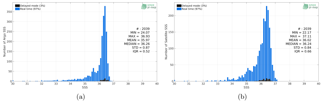
Figure 2: Histograms of SSS from Argo (a) and SMAP-L3-JPL-V4.3-8DAY-RUNNING-60KM (b) considering all match-up pairs per bins of 0.1 over the Mississippi river plume Pi-MEP region and for the full satellite product period.
