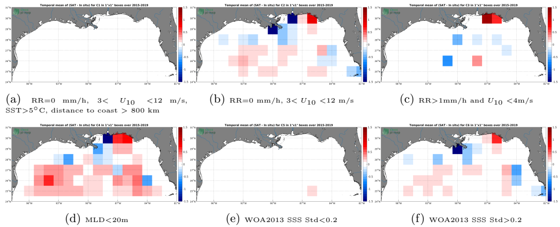
Figure 12: Temporal mean gridded over spatial boxes of size 1^\circ \times 1^\circ of \Delta SSS (SMAP-L3-JPL-V4.3-8DAY-RUNNING-60KM - Argo) for 6 different subdatasets corresponding to:RR=0 mm/h, 3 < U_{10} < 12 m/s, SST >5^\circ C, distance to coast > 800 km (a), RR=0 mm/h, 3 < U_{10} < 12 m/s (b), RR >1 mm/h and U_{10} < 4 m/s (c),MLD <20 m (d),WOA2013 SSS Std <0.2 (e),WOA2013 SSS Std >0.2 (f).
