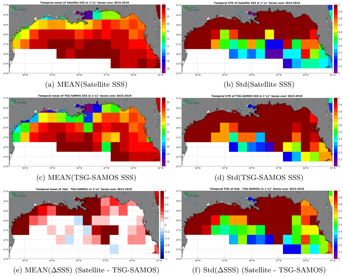
Figure 6: Temporal mean (left) and Std (right) of SSS from SMAP-L3-JPL-V4.3-MONTHLY-60KM (top), TSG-SAMOS (middle), and of \Delta SSS (Satellite - TSG-SAMOS). Only match-up pairs are used to generate these maps.
