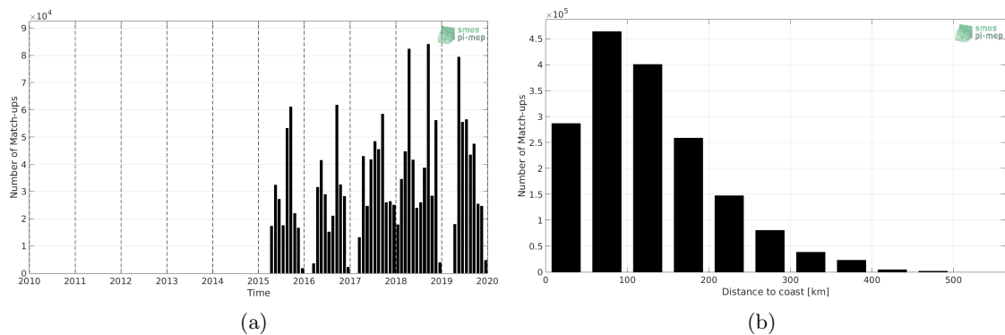
Figure 1: Number of match-ups between TSG-SAMOS and SMAP-L3-JPL-V4.3-MONTHLY-60KM SSS as a function of time (a) and as function of the distance to coast (b) over the Mississippi river plume Pi-MEP region and for the full satellite product period.
