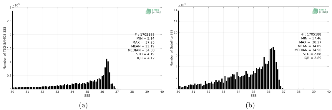
Figure 2: Histograms of SSS from TSG-SAMOS (a) and SMAP-L3-JPL-V4.3-MONTHLY-60KM (b) considering all match-up pairs per bins of 0.1 over the Mississippi river plume Pi-MEP region and for the full satellite product period.
