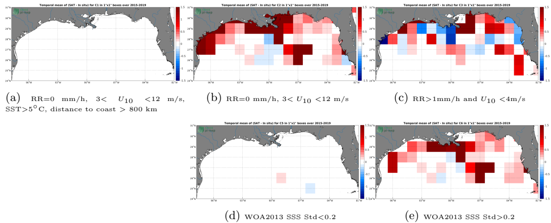
Figure 12: Temporal mean gridded over spatial boxes of size 1^{\circ}\times 1^{\circ} of \Delta\text{SSS} (SMAP-L3-JPL-V4.3-MONTHLY-60KM - TSG-SAMOS) for 5 different subdatasets corresponding to:RR=0 mm/h, 3 < U_{10} < 12 m/s, SST > 5^{\circ}\text{C} , distance to coast > 800 km (a), RR=0 mm/h, 3 < U_{10} < 12 m/s (b), RR > 1 mm/h and U_{10} < 4 m/s (c), WOA2013 SSS Std < 0.2 (d), WOA2013 SSS Std > 0.2 (e).
