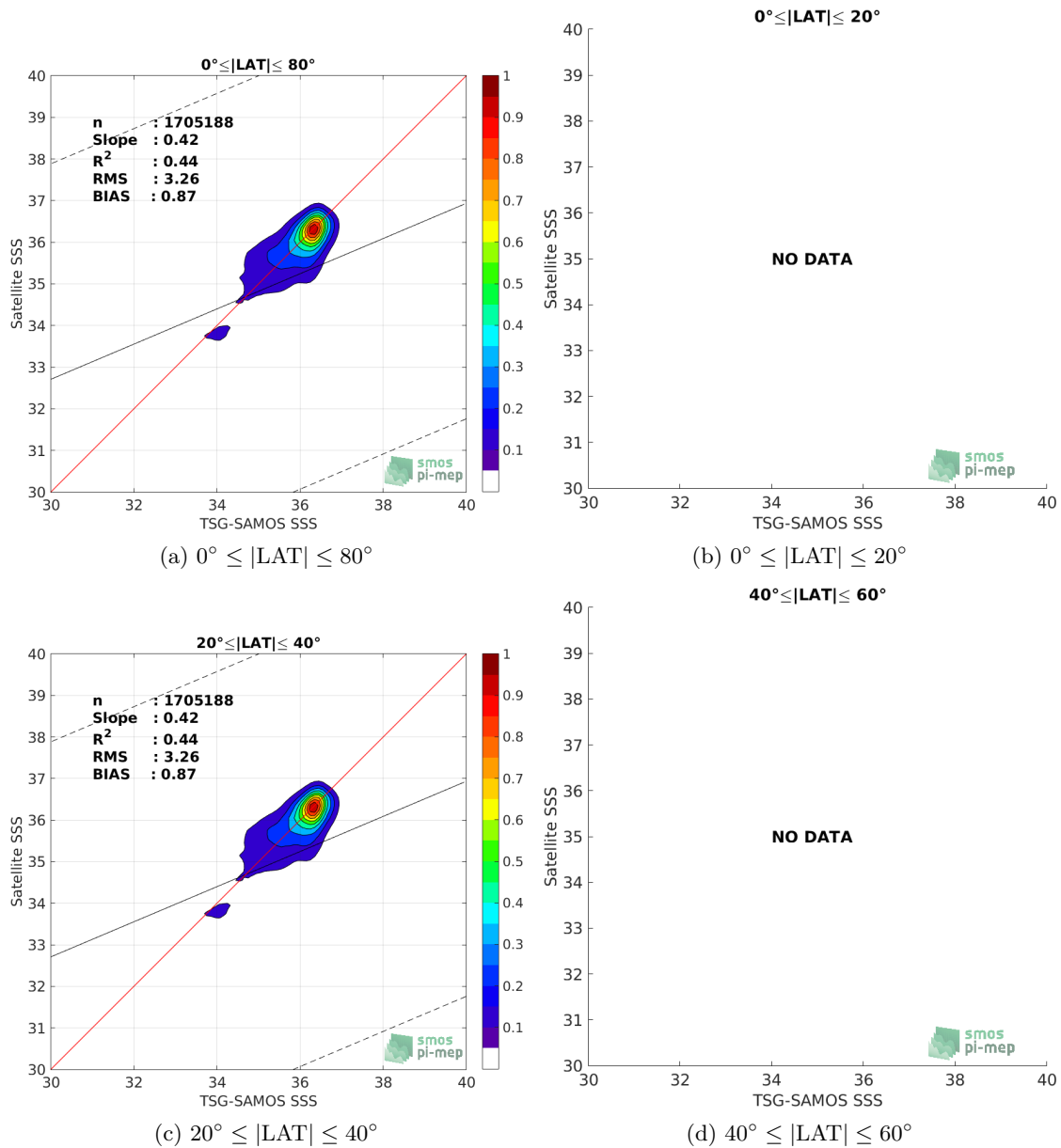
Figure 9: Contour maps of the concentration of SMAP-L3-JPL-V4.3-MONTHLY-60KM SSS (y-axis) versus TSG-SAMOS SSS (x-axis) at match-up pairs for different latitude bands. For each plot, the red line shows x=y . The black thin and dashed lines indicate a linear fit through the data cloud and the \pm 95\% confidence levels, respectively. The number match-up pairs n , the slope and R^2 coefficient of the linear fit, the root mean square (RMS) and the mean bias between satellite and in situ data are indicated for each latitude band in each plots.
