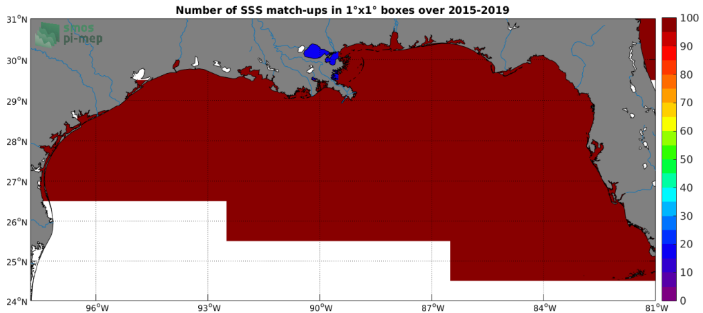
Figure 4: Number of SSS match-ups between TSG-SAMOS SSS and the SMAP-L3-JPL-V4.3-MONTHLY-60KM SSS product for the Mississippi river plume Pi-MEP region over 1°x1° boxes and for the full satellite product period.
