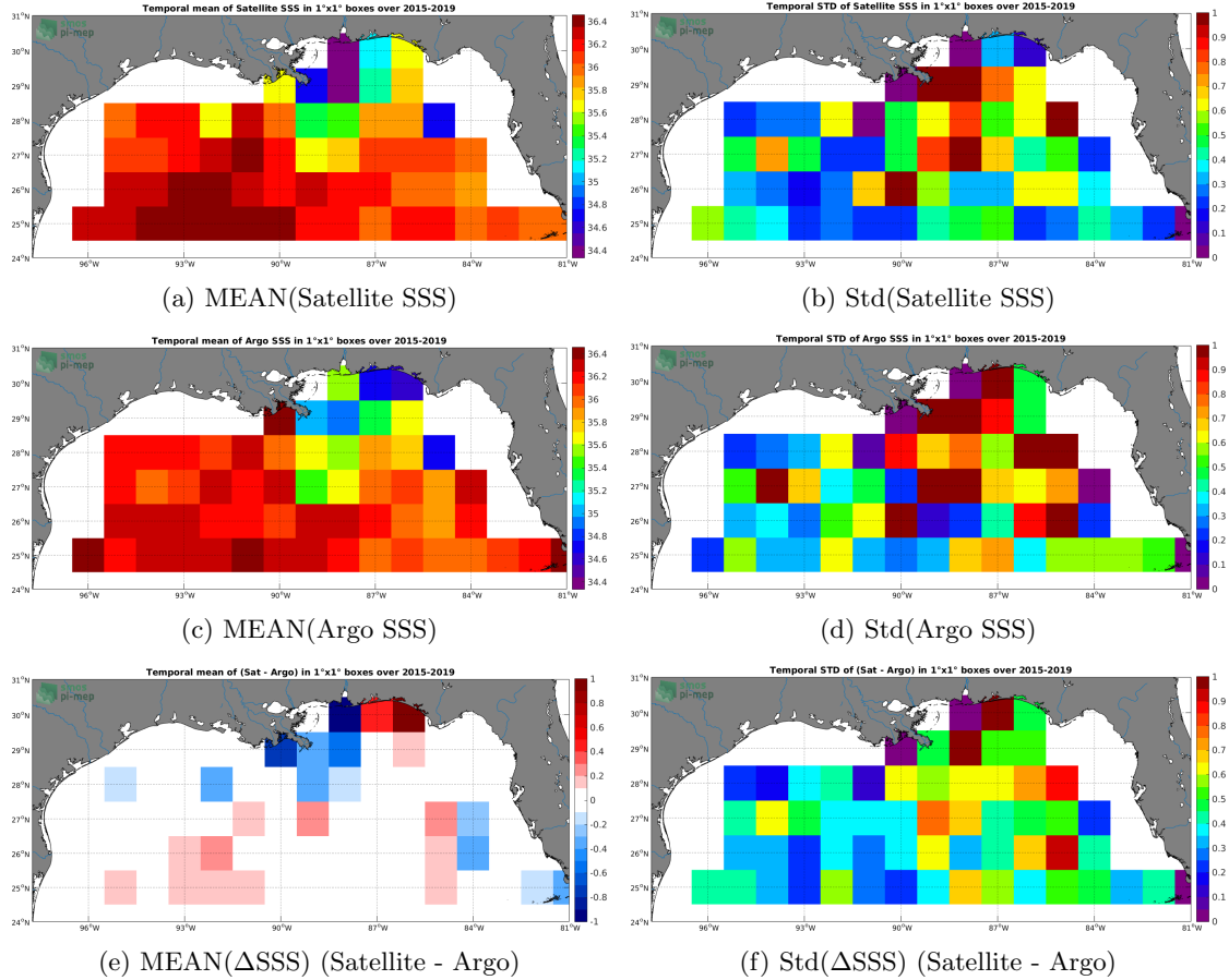
Figure 6: Temporal mean (left) and Std (right) of SSS from SMAP-L3-JPL-V4.3-MONTHLY-60KM (top), Argo (middle), and of \Delta\text{SSS} (Satellite - Argo). Only match-up pairs are used to generate these maps.
