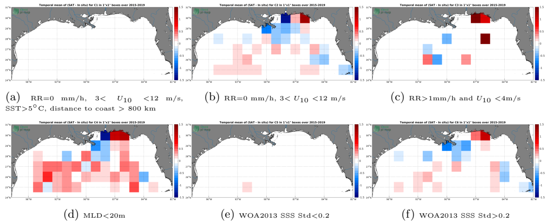
Figure 12: Temporal mean gridded over spatial boxes of size 1^\circ \times 1^\circ of \Delta SSS (SMAP-L3-JPL-V4.3-MONTHLY-60KM - Argo) for 6 different subdatasets corresponding to:RR=0 mm/h, 3 < U_{10} < 12 m/s, SST >5^\circ C, distance to coast > 800 km (a), RR=0 mm/h, 3 < U_{10} < 12 m/s (b), RR >1 mm/h and U_{10} < 4 m/s (c),MLD <20 m (d),WOA2013 SSS Std <0.2 (e),WOA2013 SSS Std >0.2 (f).
