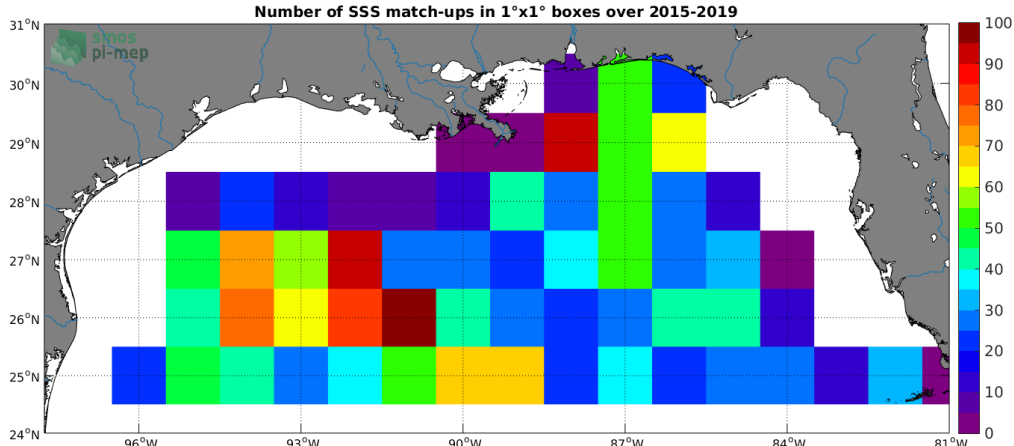
Figure 4: Number of SSS match-ups between Argo SSS and the SMAP-L3-JPL-V4.3-MONTHLY-60KM SSS product for the Mississippi river plume Pi-MEP region over 1°x1° boxes and for the full satellite product period.
