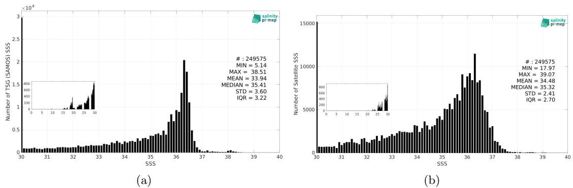
Figure 3: Histograms of SSS from TSG (SAMOS) (a) and SMAP SSS L2 v6 (RSS) (b) considering all match-up pairs per bins of 0.1 over the Mississippi river plume Pi-MEP region and for the full satellite product period.
