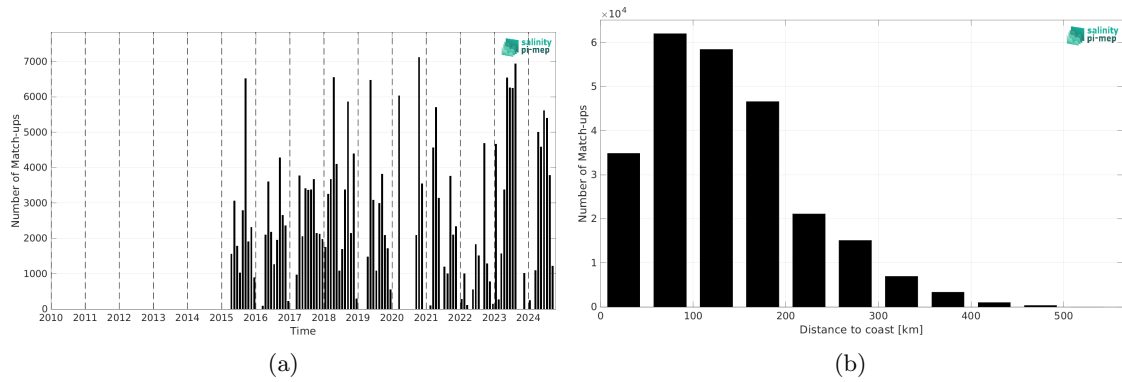
Figure 2: Number of match-ups between TSG (SAMOS) and SMAP SSS L2 v6 (RSS) SSS as a function of time (a) and as function of the distance to coast (b) over the Mississippi river plume Pi-MEP region and for the full satellite product period.
