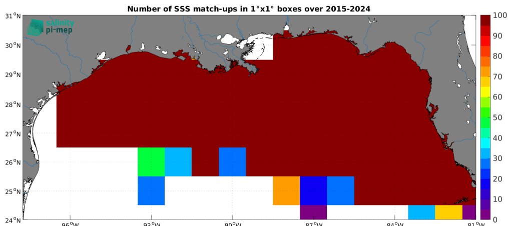
Figure 5: Number of SSS match-ups between TSG (SAMOS) SSS and the SMAP SSS L2 v6 (RSS) SSS product for the Mississippi river plume Pi-MEP region over 1^\circ \times 1^\circ boxes and for the full satellite product period.
