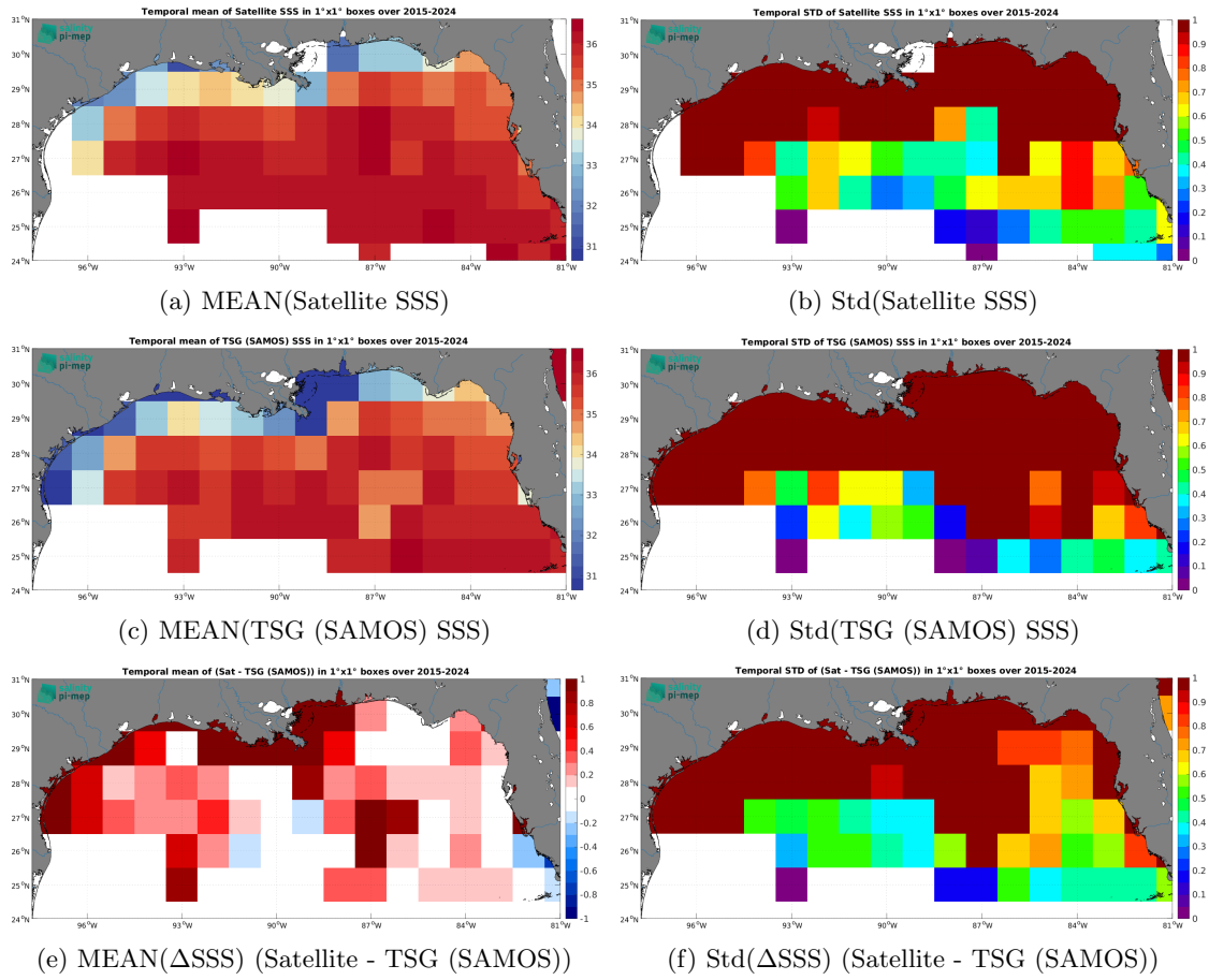
Figure 7: Temporal mean (left) and Std (right) of SSS from SMAP SSS L2 v6 (RSS) (top), TSG (SAMOS) (middle), and of \Delta SSS (Satellite - TSG (SAMOS)). Only match-up pairs are used to generate these maps.
