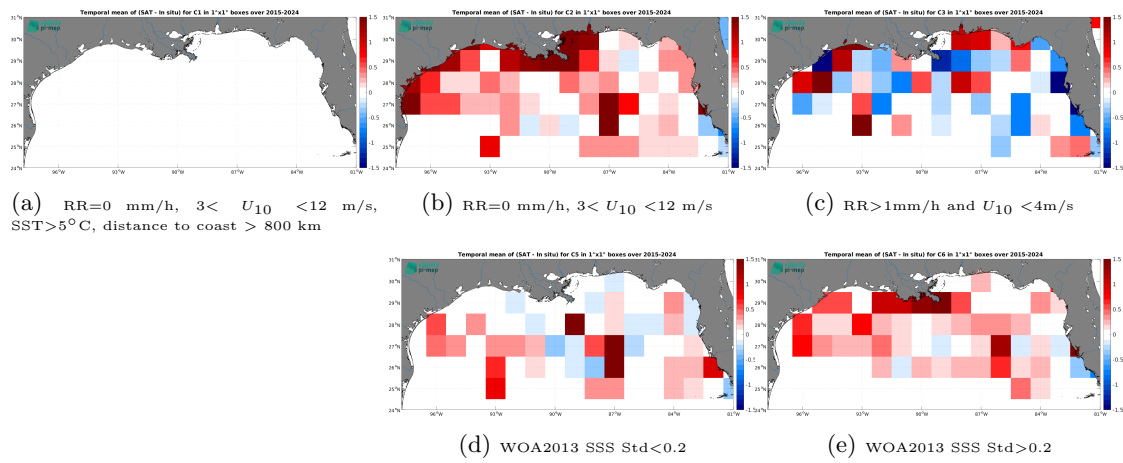
Figure 14: Temporal mean gridded over spatial boxes of size 1^\circ \times 1^\circ of \Delta SSS (SMAP SSS L2 v6 (RSS) - TSG (SAMOS)) for 5 different subdatasets corresponding to:RR=0 mm/h, 3 < U_{10} < 12 m/s, SST > 5°C, distance to coast > 800 km (a), RR=0 mm/h, 3 < U_{10} < 12 m/s (b), RR > 1mm/h and U_{10} < 4 m/s (c), WOA2013 SSS Std < 0.2 (d), WOA2013 SSS Std > 0.2 (e).
