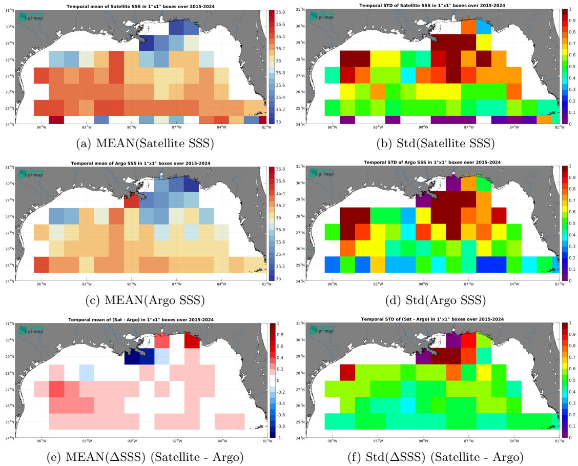
Figure 7: Temporal mean (left) and Std (right) of SSS from SMAP SSS L2 v6 (RSS) (top), Argo (middle), and of \Delta SSS (Satellite - Argo). Only match-up pairs are used to generate these maps.
