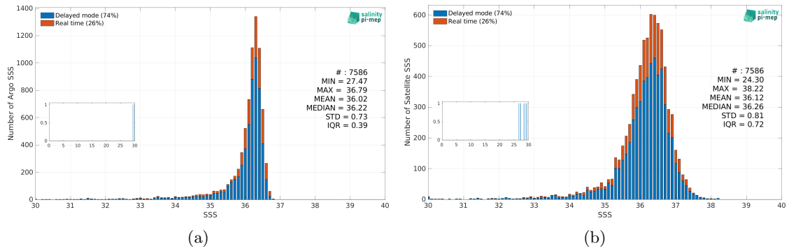
Figure 3: Histograms of SSS from Argo (a) and SMAP SSS L2 v6 (RSS) (b) considering all match-up pairs per bins of 0.1 over the Mississippi river plume Pi-MEP region and for the full satellite product period.
