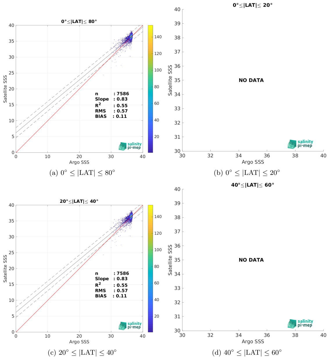
Figure 10: Contour maps of the concentration of SMAP SSS L2 v6 (RSS) SSS (y-axis) versus Argo SSS (x-axis) at match-up pairs for different latitude bands. For each plot, the red line shows x=y . The black thin and dashed lines indicate a linear fit through the data cloud and the \pm 95\% confidence levels, respectively. The number match-up pairs n , the slope and R^2 coefficient of the linear fit, the root mean square (RMS) and the mean bias between satellite and in situ data are indicated for each latitude band in each plots.
