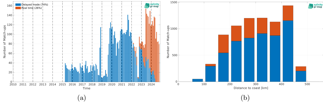
Figure 2: Number of match-ups between Argo and SMAP SSS L2 v6 (RSS) SSS as a function of time (a) and as function of the distance to coast (b) over the Mississippi river plume Pi-MEP region and for the full satellite product period.
