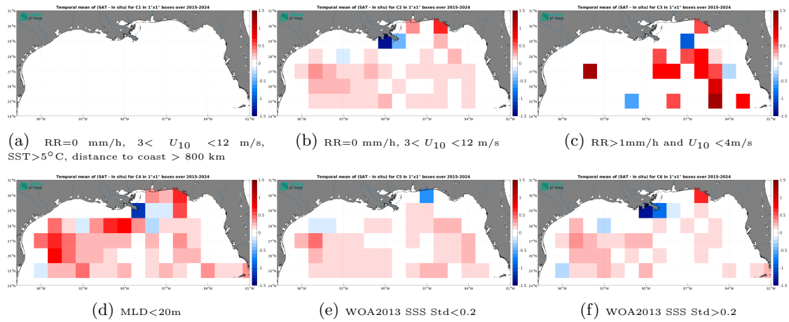
Figure 14: Temporal mean gridded over spatial boxes of size 1^\circ \times 1^\circ of \Delta SSS (SMAP SSS L2 v6 (RSS) - Argo) for 6 different subdatasets corresponding to:RR=0 mm/h, 3 < U_{10} < 12 m/s, SST >5^\circ\text{C} , distance to coast > 800 km (a), RR=0 mm/h, 3 < U_{10} < 12 m/s (b), RR >1 mm/h and U_{10} < 4 m/s (c),MLD <20 m (d),WOA2013 SSS Std <0.2 (e),WOA2013 SSS Std >0.2 (f).
