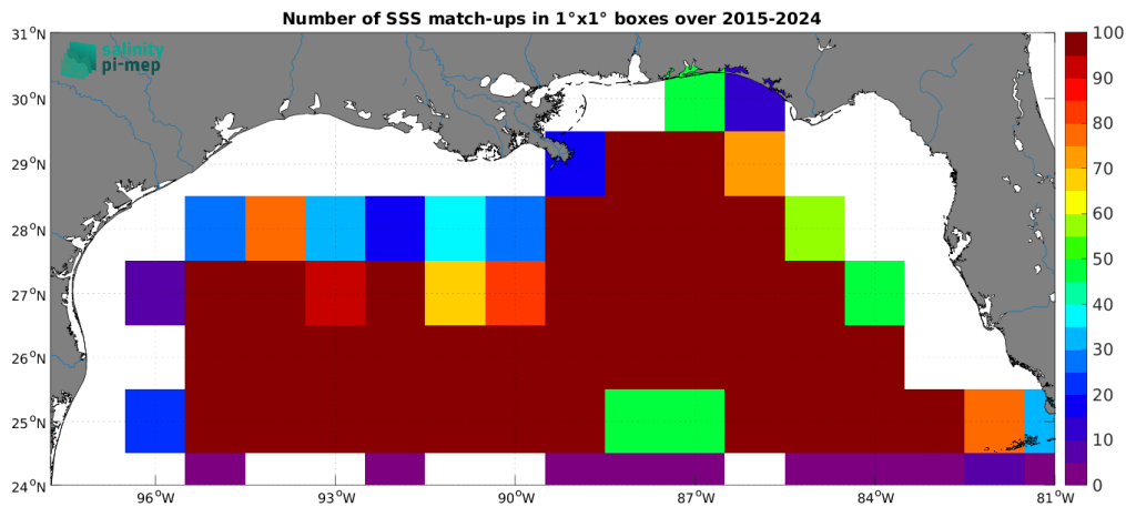
Figure 5: Number of SSS match-ups between Argo SSS and the SMAP SSS L2 v6 (RSS) SSS product for the Mississippi river plume Pi-MEP region over 1^\circ \times 1^\circ boxes and for the full satellite product period.
