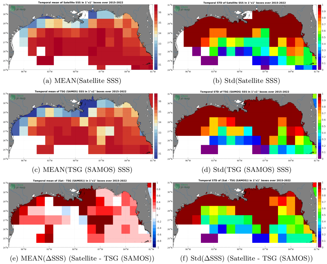
Figure 6: Temporal mean (left) and Std (right) of SSS from SMAP SSS L2 v5 (RSS) (top), TSG (SAMOS) (middle), and of \Delta SSS (Satellite - TSG (SAMOS)). Only match-up pairs are used to generate these maps.
