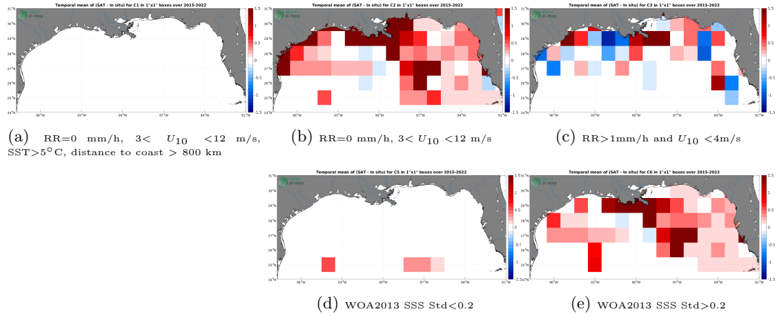
Figure 12: Temporal mean gridded over spatial boxes of size 1^{\circ}\times 1^{\circ} of \Delta\text{SSS} (SMAP SSS L2 v5 (RSS) - TSG (SAMOS)) for 5 different subdatasets corresponding to:RR=0 mm/h, 3 < U_{10} < 12 m/s, SST > 5^{\circ}\text{C} , distance to coast > 800 km (a), RR=0 mm/h, 3 < U_{10} < 12 m/s (b), RR > 1 mm/h and U_{10} < 4 m/s (c), WOA2013 SSS Std < 0.2 (d), WOA2013 SSS Std > 0.2 (e).
