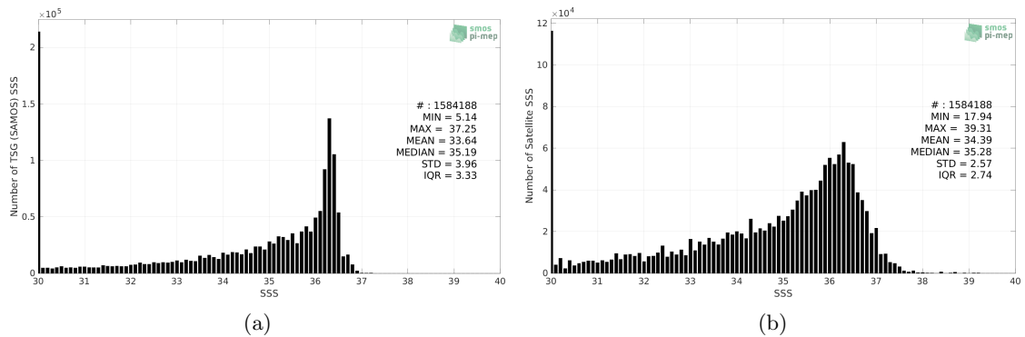
Figure 2: Histograms of SSS from TSG (SAMOS) (a) and SMAP SSS L2 v5 (RSS) (b) considering all match-up pairs per bins of 0.1 over the Mississippi river plume Pi-MEP region and for the full satellite product period.
