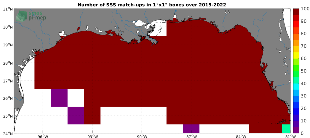
Figure 4: Number of SSS match-ups between TSG (SAMOS) SSS and the SMAP SSS L2 v5 (RSS) SSS product for the Mississippi river plume Pi-MEP region over 1^\circ \times 1^\circ boxes and for the full satellite product period.
