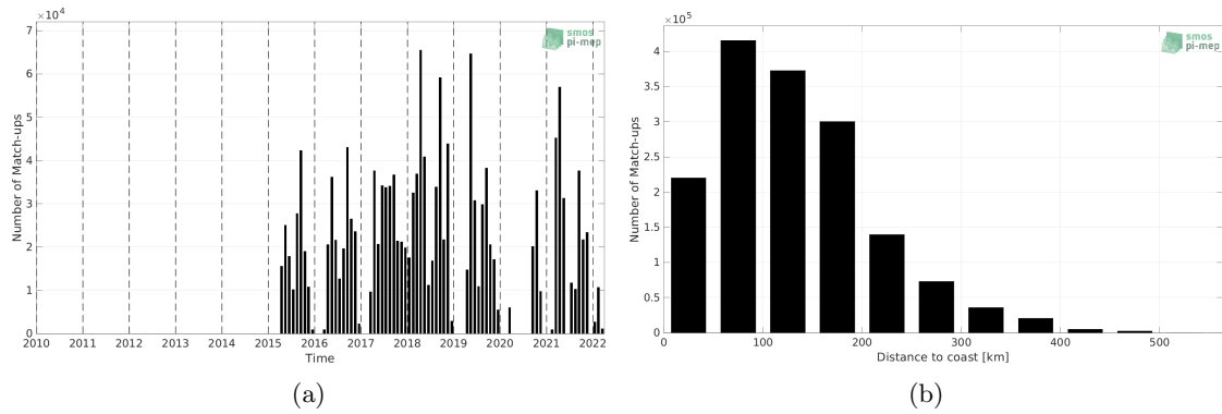
Figure 1: Number of match-ups between TSG (SAMOS) and SMAP SSS L2 v5 (RSS) SSS as a function of time (a) and as function of the distance to coast (b) over the Mississippi river plume Pi-MEP region and for the full satellite product period.
