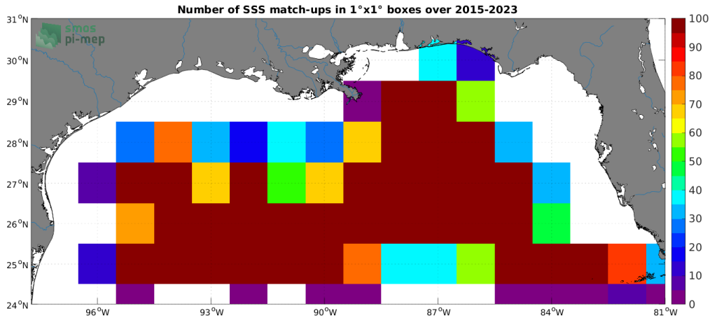
Figure 4: Number of SSS match-ups between Argo SSS and the SMAP SSS L2 v5 (RSS) SSS product for the Mississippi river plume Pi-MEP region over 1^{\circ} \times 1^{\circ} boxes and for the full satellite product period.
