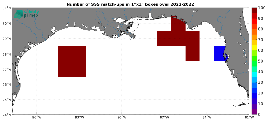
Figure 5: Number of SSS match-ups between Saildrone SSS and the SMAP SSS L2 v5.3 - 40 km (RSS) SSS product for the Mississippi river plume Pi-MEP region over 1^{\circ} \times 1^{\circ} boxes and for the full satellite product period.
