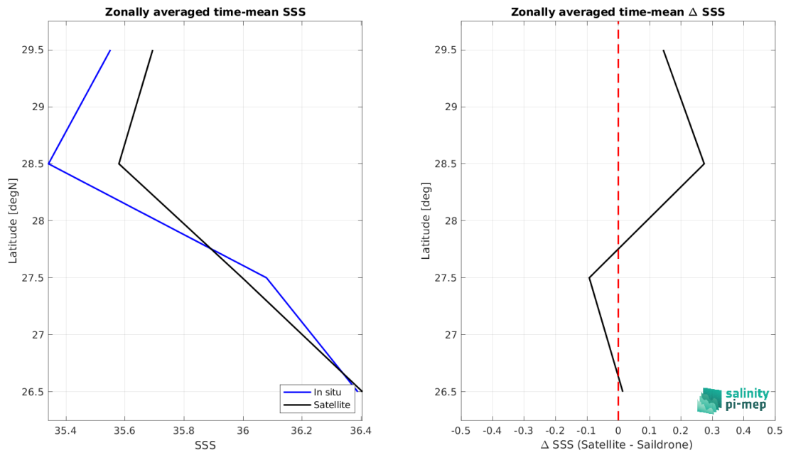
Figure 9: Left panel: Zonal mean SSS from SMAP SSS L2 v5.3 - 40 km (RSS) satellite product (black) and from Sairdrone (blue). Right panel: Zonal mean of \Delta SSS (Satellite - Sairdrone) for all the collected Pi-MEP match-up pairs estimated over the full satellite product period.
