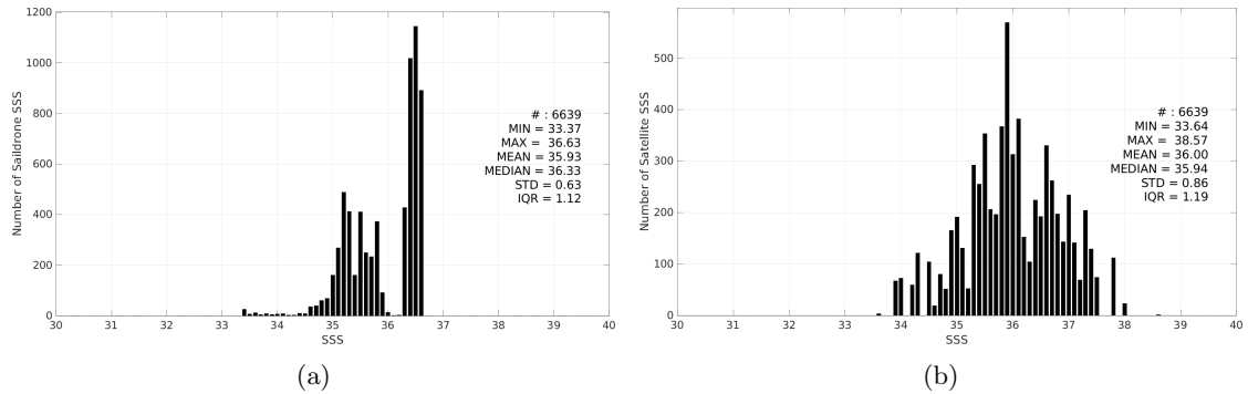
Figure 3: Histograms of SSS from Saildrone (a) and SMAP SSS L2 v5.3 - 40 km (RSS) (b) considering all match-up pairs per bins of 0.1 over the Mississippi river plume Pi-MEP region and for the full satellite product period.
