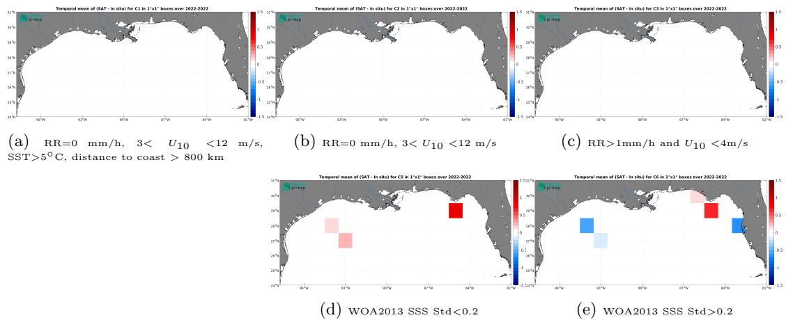
Figure 14: Temporal mean gridded over spatial boxes of size 1^\circ \times 1^\circ of \Delta SSS (SMAP SSS L2 v5.3 - 40 km (RSS) - Sailability) for 5 different subdatasets corresponding to:RR=0 mm/h, 3 < U_{10} < 12 m/s, SST > 5°C, distance to coast > 800 km (a), RR=0 mm/h, 3 < U_{10} < 12 m/s (b), RR > 1mm/h and U_{10} < 4 m/s (c), WOA2013 SSS Std < 0.2 (d), WOA2013 SSS Std > 0.2 (e).
