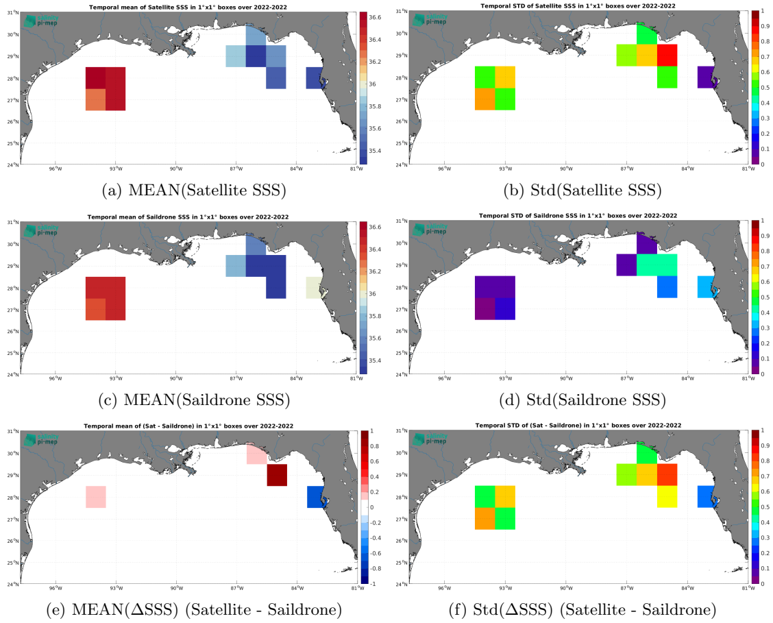
Figure 7: Temporal mean (left) and Std (right) of SSS from SMAP SSS L2 v5.3 - 40 km (RSS) (top), Saildrone (middle), and of \Delta SSS (Satellite - Saildrone). Only match-up pairs are used to generate these maps.
