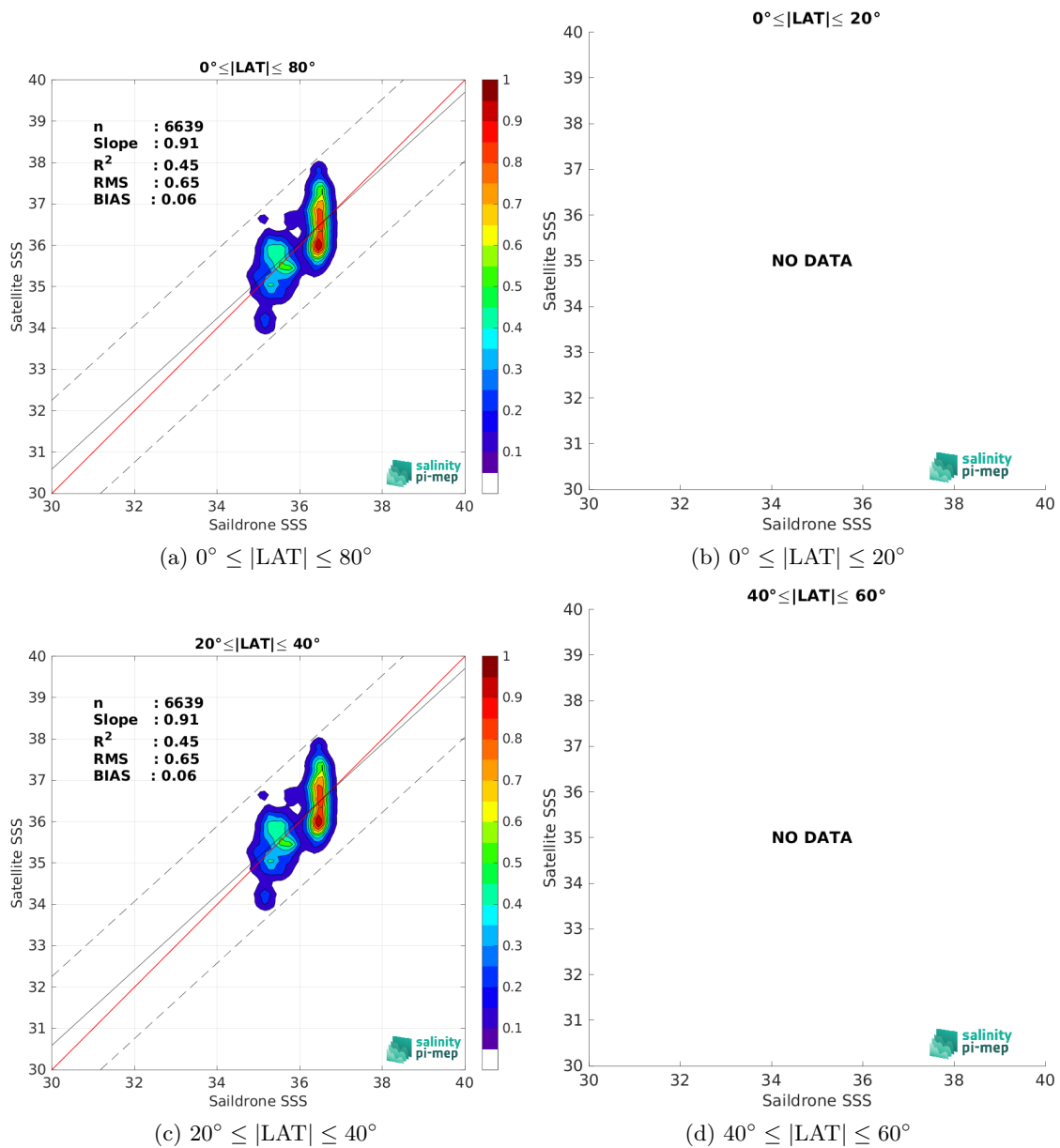
Figure 10: Contour maps of the concentration of SMAP SSS L2 v5.3 - 40 km (RSS) SSS (y-axis) versus Saïdrone SSS (x-axis) at match-up pairs for different latitude bands. For each plot, the red line shows x=y . The black thin and dashed lines indicate a linear fit through the data cloud and the \pm 95\% confidence levels, respectively. The number match-up pairs n , the slope and R^2 coefficient of the linear fit, the root mean square (RMS) and the mean bias between satellite and in situ data are indicated for each latitude band in each plots.
