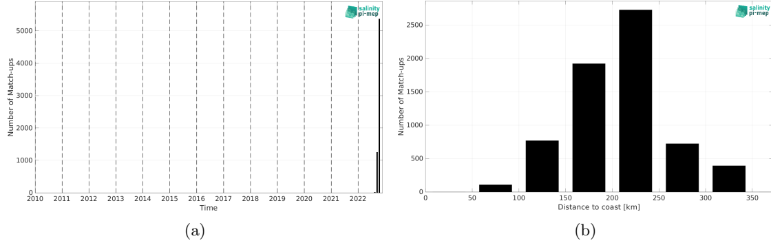
Figure 2: Number of match-ups between Saildrone and SMAP SSS L2 v5.3 - 40 km (RSS) SSS as a function of time (a) and as function of the distance to coast (b) over the Mississippi river plume Pi-MEP region and for the full satellite product period.
