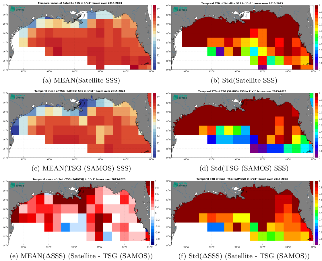
Figure 6: Temporal mean (left) and Std (right) of SSS from SMAP SSS L2 v5 - 40 km (RSS) (top), TSG (SAMOS) (middle), and of \Delta SSS (Satellite - TSG (SAMOS)). Only match-up pairs are used to generate these maps.
