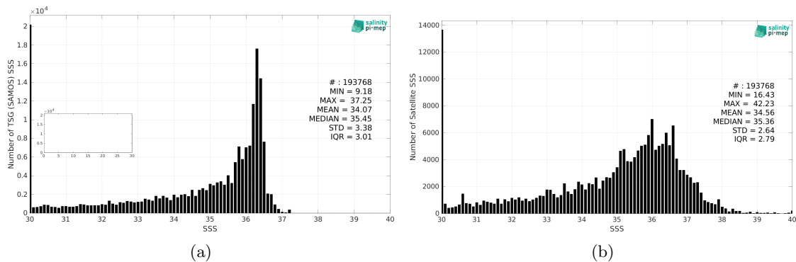
Figure 2: Histograms of SSS from TSG (SAMOS) (a) and SMAP SSS L2 v5 - 40 km (RSS) (b) considering all match-up pairs per bins of 0.1 over the Mississippi river plume Pi-MEP region and for the full satellite product period.
