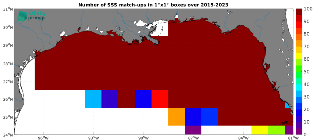
Figure 4: Number of SSS match-ups between TSG (SAMOS) SSS and the SMAP SSS L2 v5 - 40 km (RSS) SSS product for the Mississippi river plume Pi-MEP region over 1^\circ \times 1^\circ boxes and for the full satellite product period.
