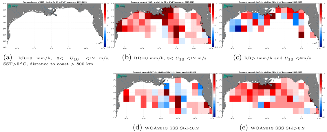
Figure 12: Temporal mean gridded over spatial boxes of size 1^{\circ}\times 1^{\circ} of \Delta\text{SSS} (SMAP SSS L2 v5 - 40 km (RSS) - TSG (SAMOS)) for 5 different subdatasets corresponding to:RR=0 mm/h, 3 < U_{10} < 12 m/s, SST >5^{\circ}\text{C} , distance to coast > 800 km (a), RR=0 mm/h, 3 < U_{10} < 12 m/s (b), RR >1 mm/h and U_{10} < 4 m/s (c), WOA2013 SSS Std <0.2 (d), WOA2013 SSS Std >0.2 (e).
