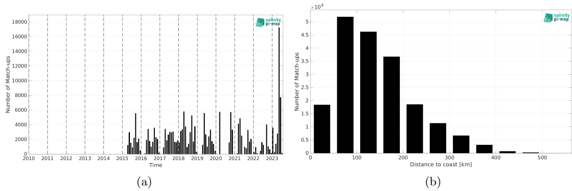
Figure 1: Number of match-ups between TSG (SAMOS) and SMAP SSS L2 v5 - 40 km (RSS) SSS as a function of time (a) and as function of the distance to coast (b) over the Mississippi river plume Pi-MEP region and for the full satellite product period.
