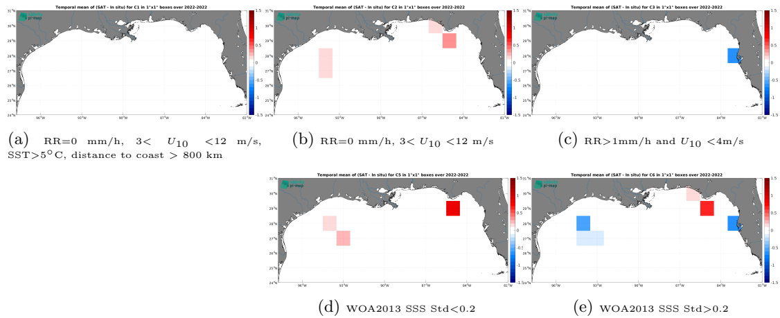
Figure 12: Temporal mean gridded over spatial boxes of size 1^{\circ}\times 1^{\circ} of \Delta\text{SSS} (SMAP SSS L2 v5 - 40 km (RSS) - Saildrone) for 5 different subdatasets corresponding to:RR=0 mm/h, 3 < U_{10} < 12 m/s, SST >5^{\circ}\text{C} , distance to coast > 800 km (a), RR=0 mm/h, 3 < U_{10} < 12 m/s (b), RR >1 mm/h and U_{10} < 4 m/s (c), WOA2013 SSS Std <0.2 (d), WOA2013 SSS Std >0.2 (e).
