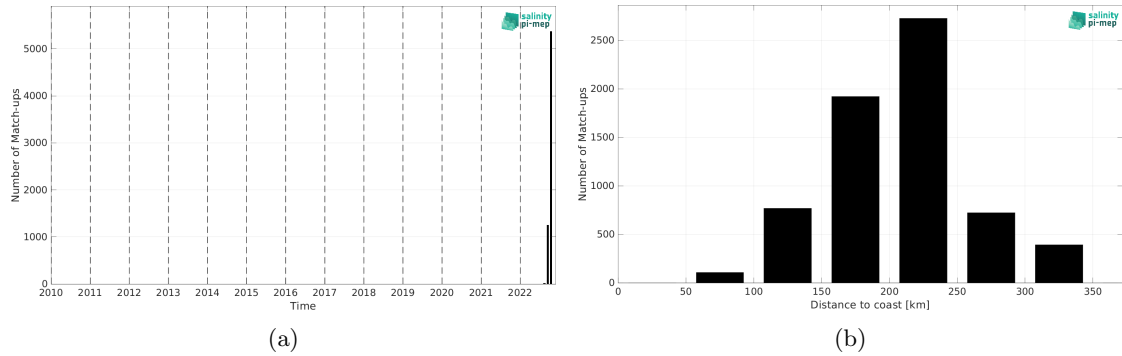
Figure 1: Number of match-ups between Sairdrone and SMAP SSS L2 v5 - 40 km (RSS) SSS as a function of time (a) and as function of the distance to coast (b) over the Mississippi river plume Pi-MEP region and for the full satellite product period.
