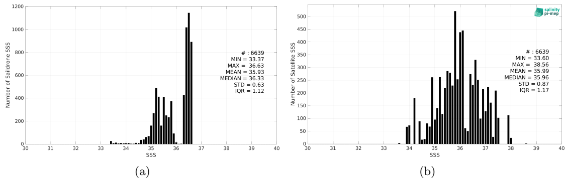
Figure 2: Histograms of SSS from Sairdrone (a) and SMAP SSS L2 v5 - 40 km (RSS) (b) considering all match-up pairs per bins of 0.1 over the Mississippi river plume Pi-MEP region and for the full satellite product period.
