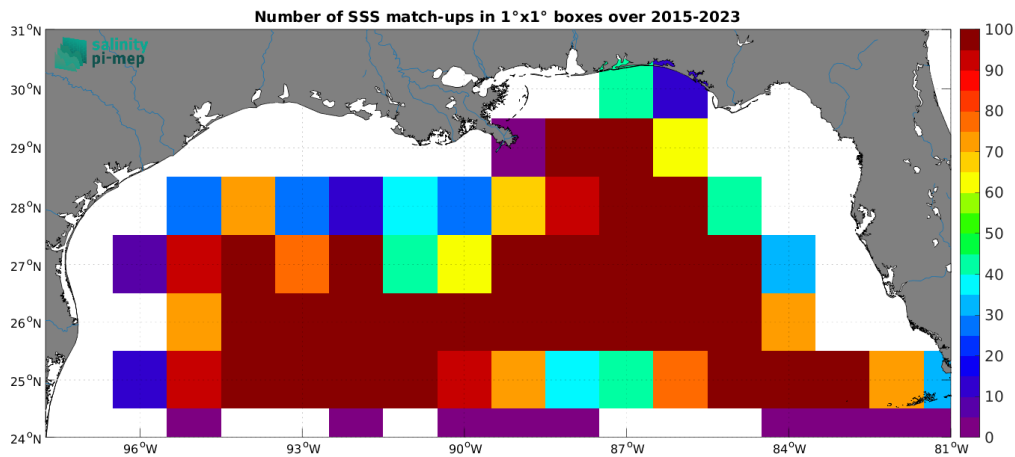
Figure 4: Number of SSS match-ups between Argo SSS and the SMAP SSS L2 v5 - 40 km (RSS) SSS product for the Mississippi river plume Pi-MEP region over 1^\circ \times 1^\circ boxes and for the full satellite product period.
