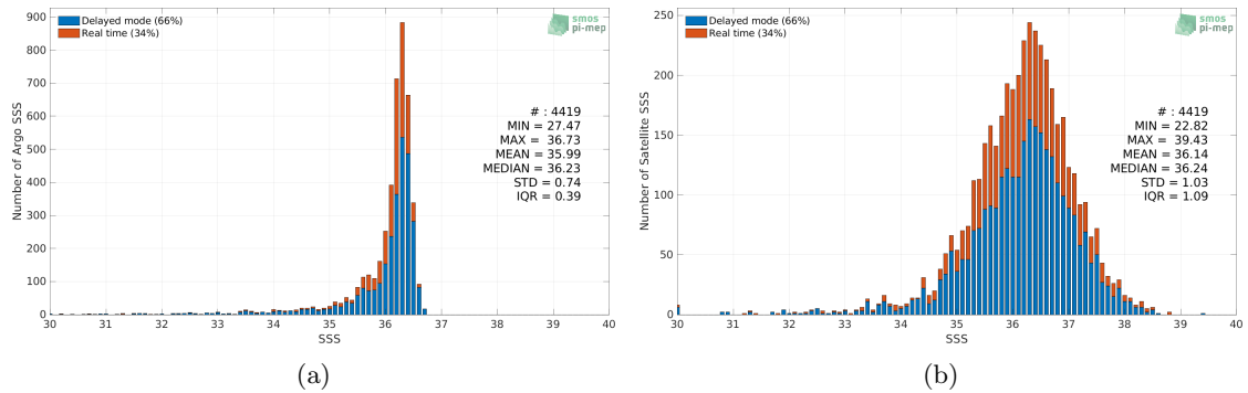
Figure 2: Histograms of SSS from Argo (a) and SMAP SSS L2 v5 - 40 km (RSS) (b) considering all match-up pairs per bins of 0.1 over the Mississippi river plume Pi-MEP region and for the full satellite product period.
