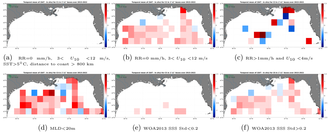
Figure 12: Temporal mean gridded over spatial boxes of size 1^{\circ}\times 1^{\circ} of \Delta\text{SSS} (SMAP SSS L2 v5 - 40 km (RSS) - Argo) for 6 different subdatasets corresponding to:RR=0 mm/h, 3 < U_{10} < 12 m/s, SST > 5^{\circ}\text{C} , distance to coast > 800 km (a), RR=0 mm/h, 3 < U_{10} < 12 m/s (b), RR > 1 mm/h and U_{10} < 4 m/s (c),MLD < 20\text{m} (d),WOA2013 SSS Std < 0.2 (e),WOA2013 SSS Std > 0.2 (f).
