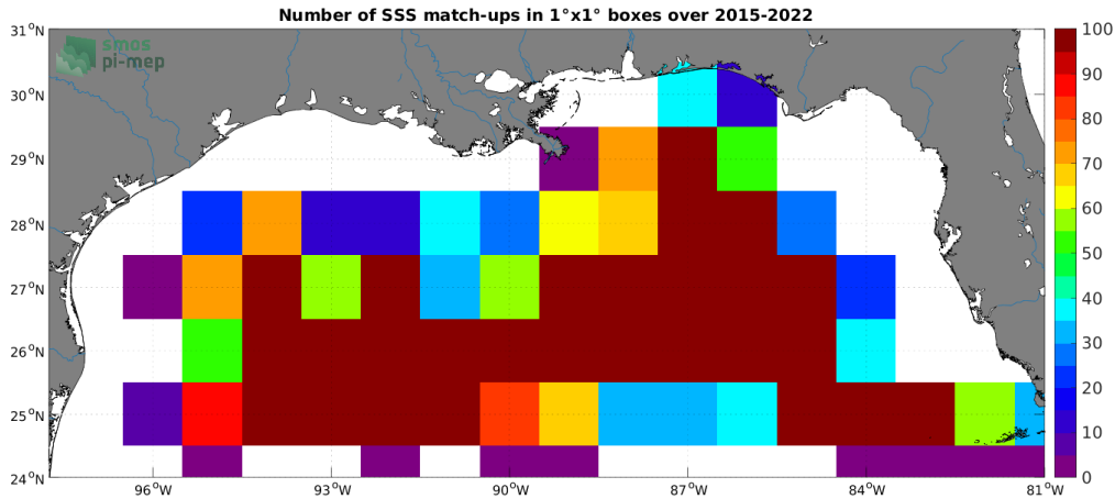
Figure 4: Number of SSS match-ups between Argo SSS and the SMAP SSS L2 v5 - 40 km (RSS) SSS product for the Mississippi river plume Pi-MEP region over 1^{\circ} \times 1^{\circ} boxes and for the full satellite product period.
