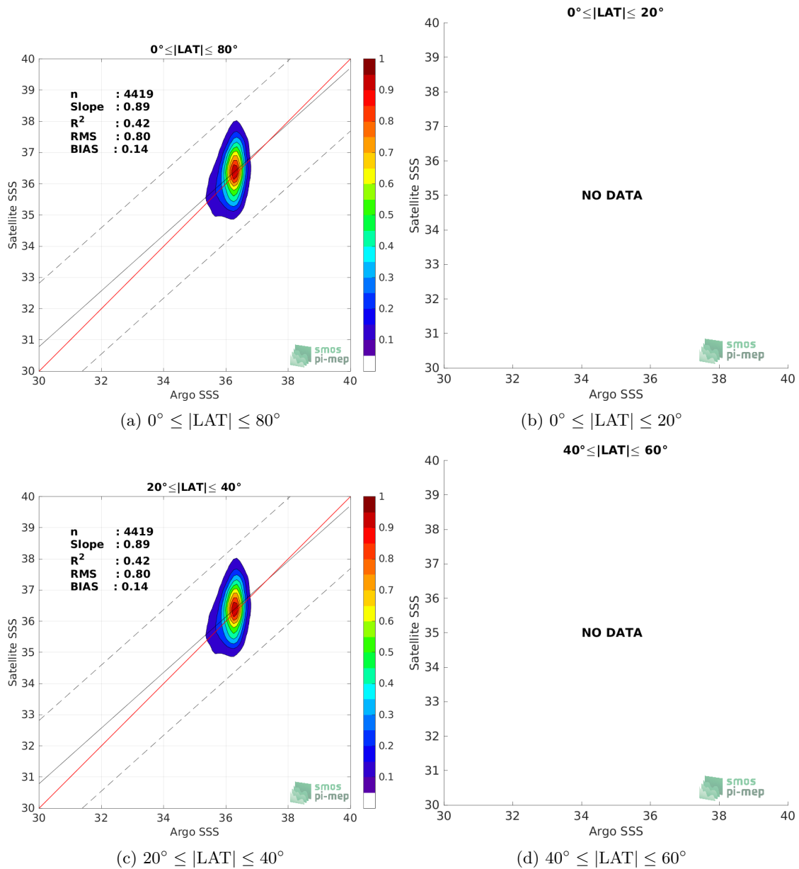
Figure 9: Contour maps of the concentration of SMAP SSS L2 v5 - 40 km (RSS) SSS (y-axis) versus Argo SSS (x-axis) at match-up pairs for different latitude bands. For each plot, the red line shows x=y . The black thin and dashed lines indicate a linear fit through the data cloud and the \pm 95\% confidence levels, respectively. The number match-up pairs n , the slope and R^2 coefficient of the linear fit, the root mean square (RMS) and the mean bias between satellite and in situ data are indicated for each latitude band in each plots.
