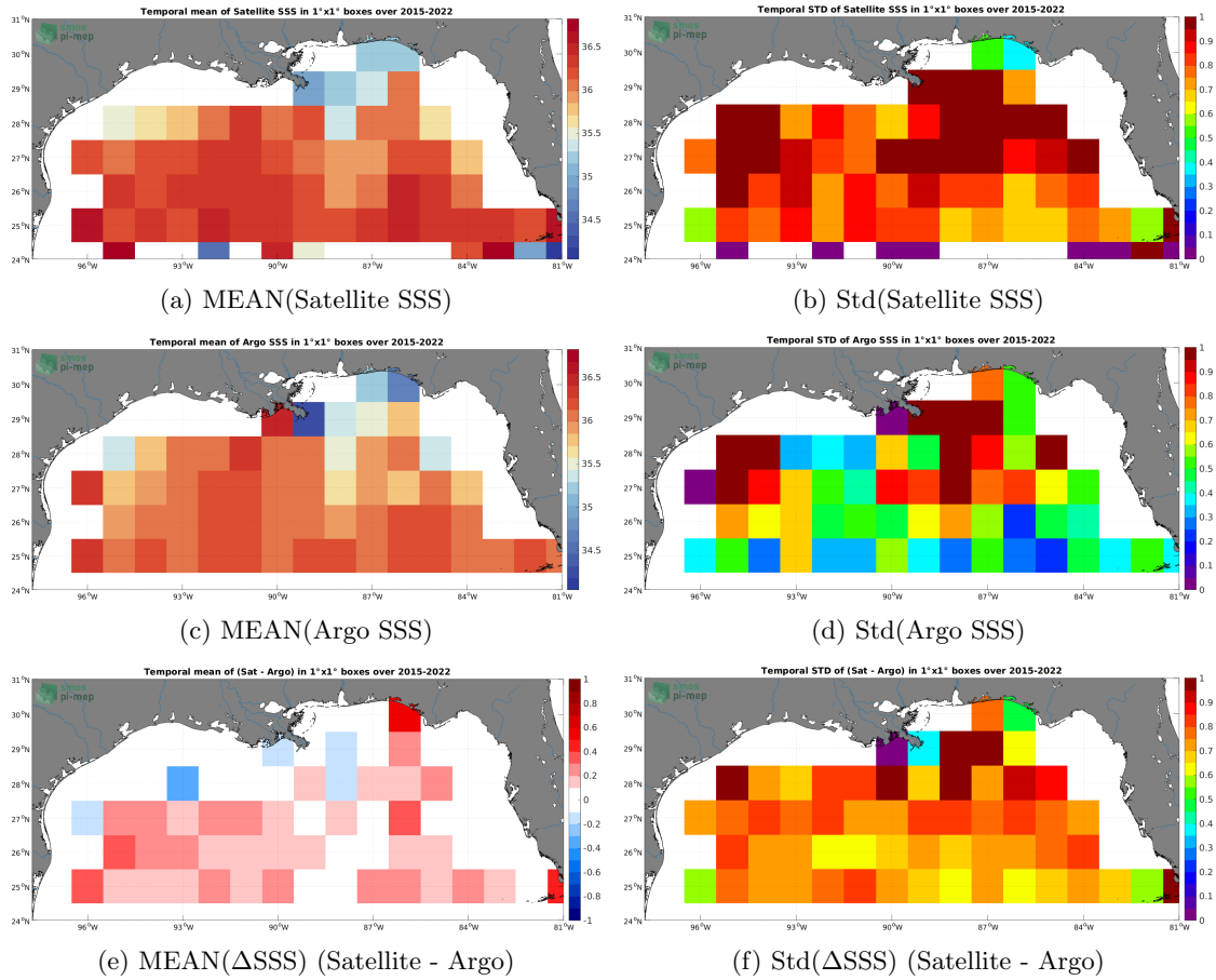
Figure 6: Temporal mean (left) and Std (right) of SSS from SMAP SSS L2 v5 - 40 km (RSS) (top), Argo (middle), and of \Delta SSS (Satellite - Argo). Only match-up pairs are used to generate these maps.
