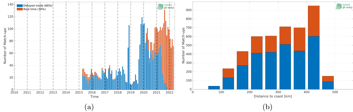
Figure 1: Number of match-ups between Argo and SMAP SSS L2 v5 - 40 km (RSS) SSS as a function of time (a) and as function of the distance to coast (b) over the Mississippi river plume Pi-MEP region and for the full satellite product period.
