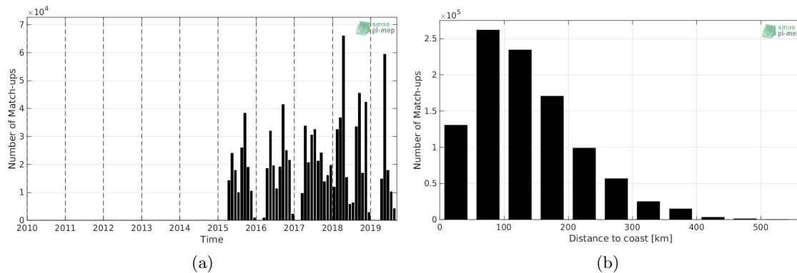
Figure 1: Number of match-ups between TSG-SAMOS and SMAP-L2-RSS-V4 SSS as a function of time (a) and as function of the distance to coast (b) over the Mississippi river plume Pi-MEP region and for the full satellite product period.
