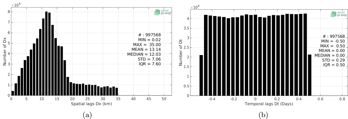
Figure 5: Histograms of the spatial (a) and temporal (b) lags between the time of the TSG-SAMOS measurements and the date of the corresponding SMAP-L2-RSS-V4 SSS product.
