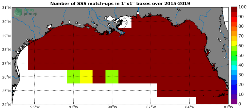
Figure 4: Number of SSS match-ups between TSG-SAMOS SSS and the SMAP-L2-RSS-V4 SSS product for the Mississippi river plume Pi-MEP region over 1°x1° boxes and for the full satellite product period.
