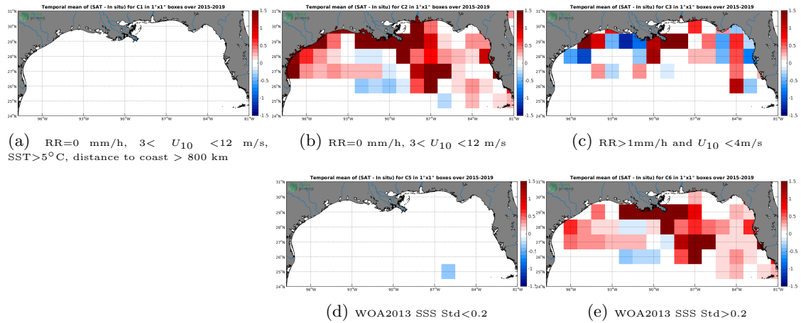
Figure 12: Temporal mean gridded over spatial boxes of size 1^\circ \times 1^\circ of \Delta SSS (SMAP-L2-RSS-V4 - TSG-SAMOS) for 5 different subdatasets corresponding to:RR=0 mm/h, 3 < U_{10} < 12 m/s, SST >5^\circ C, distance to coast > 800 km (a), RR=0 mm/h, 3 < U_{10} < 12 m/s (b), RR >1 mm/h and U_{10} < 4 m/s (c), WOA2013 SSS Std <0.2 (d), WOA2013 SSS Std >0.2 (e).
