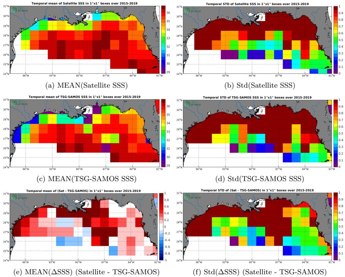
Figure 6: Temporal mean (left) and Std (right) of SSS from SMAP-L2-RSS-V4 (top), TSG-SAMOS (middle), and of \Delta SSS (Satellite - TSG-SAMOS). Only match-up pairs are used to generate these maps.
