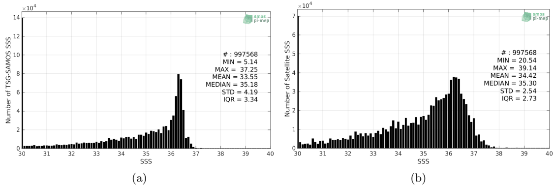
Figure 2: Histograms of SSS from TSG-SAMOS (a) and SMAP-L2-RSS-V4 (b) considering all match-up pairs per bins of 0.1 over the Mississippi river plume Pi-MEP region and for the full satellite product period.
