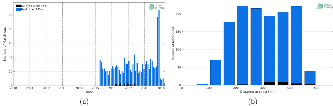
Figure 1: Number of match-ups between Argo and SMAP-L2-RSS-V3-70KM SSS as a function of time (a) and as function of the distance to coast (b) over the Mississippi river plume Pi-MEP region and for the full satellite product period.
