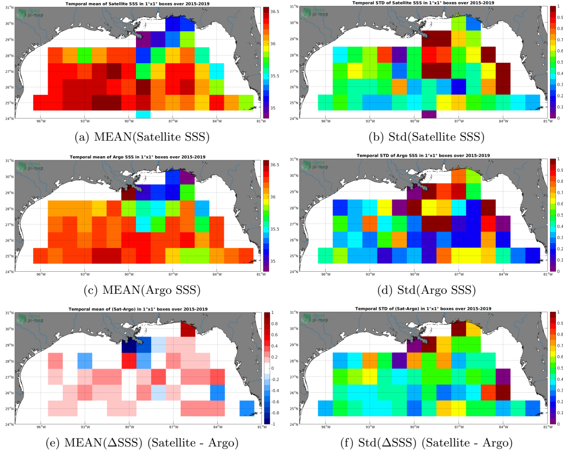
Figure 6: Temporal mean (left) and Std (right) of SSS from SMAP-L2-RSS-V3-70KM (top), Argo (middle), and of \Delta SSS (Satellite - Argo). Only match-up pairs are used to generate these maps.
