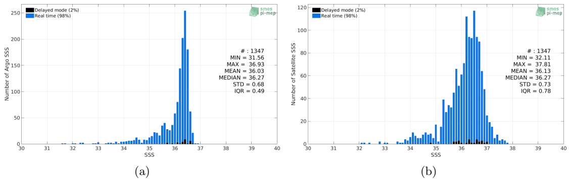
Figure 2: Histograms of SSS from Argo (a) and SMAP-L2-RSS-V3-70KM (b) considering all match-up pairs per bins of 0.1 over the Mississippi river plume Pi-MEP region and for the full satellite product period.
