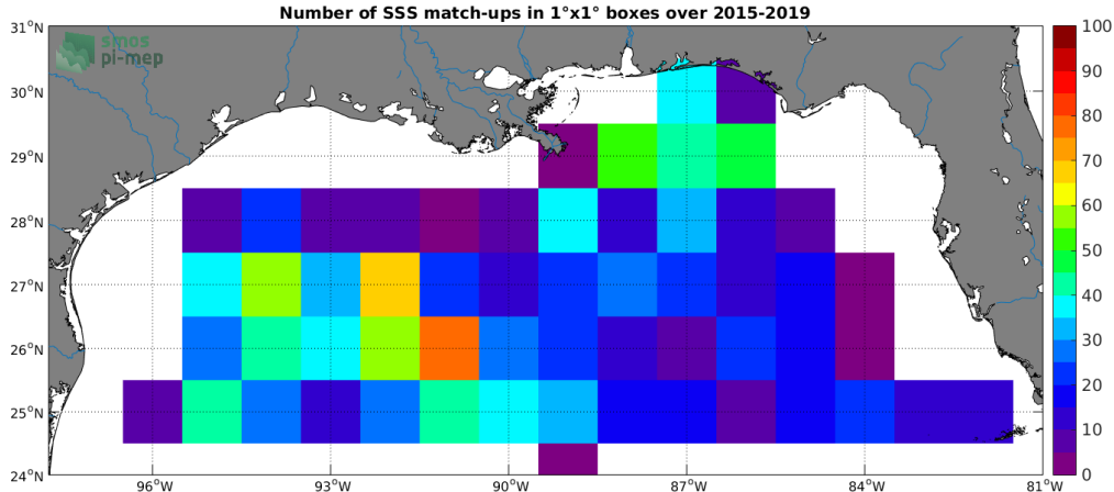
Figure 4: Number of SSS match-ups between Argo SSS and the SMAP-L2-RSS-V3-70KM SSS product for the Mississippi river plume Pi-MEP region over 1°x1° boxes and for the full satellite product period.
