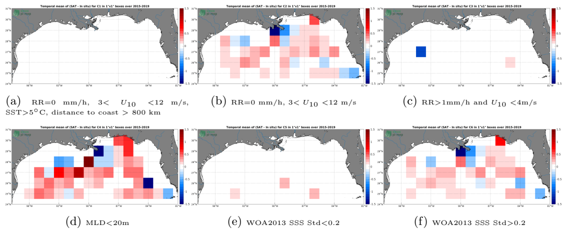
Figure 12: Temporal mean gridded over spatial boxes of size 1^\circ \times 1^\circ of \Delta SSS (SMAP-L2-RSS-V3-70KM - Argo) for 6 different subdatasets corresponding to:RR=0 mm/h, 3 < U_{10} < 12 m/s, SST >5^\circ C, distance to coast > 800 km (a), RR=0 mm/h, 3 < U_{10} < 12 m/s (b), RR >1 mm/h and U_{10} < 4 m/s (c),MLD <20 m (d),WOA2013 SSS Std <0.2 (e),WOA2013 SSS Std >0.2 (f).
