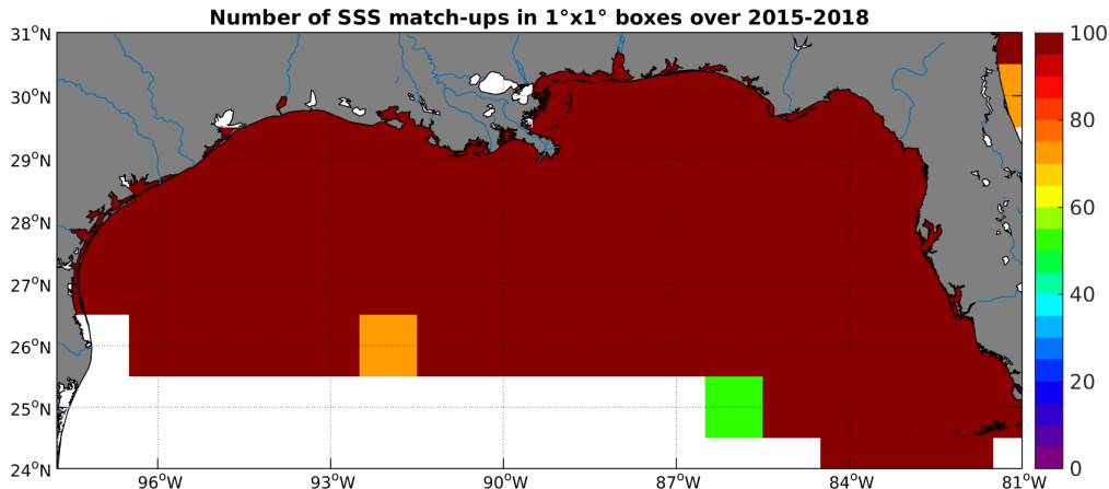
Figure 4: Number of SSS match-ups between TSG-SAMOS SSS and the SMAP-L2-JPL-V4 SSS product for the Mississippi river plume Pi-MEP region over 1^\circ \times 1^\circ boxes and for the full satellite product period.
