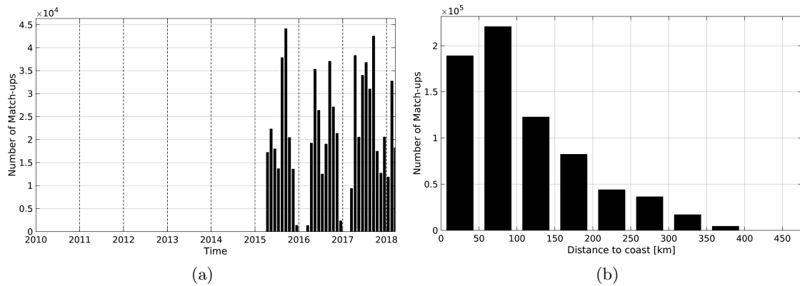
Figure 1: Number of match-ups between TSG-SAMOS and SMAP-L2-JPL-V4 SSS as a function of time (a) and as function of the distance to coast (b) over the Mississippi river plume Pi-MEP region and for the full satellite product period.
