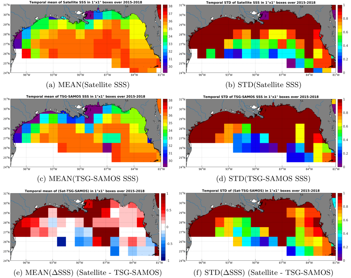
Figure 6: Temporal mean (left) and STD (right) of SSS from SMAP-L2-JPL-V4 (top), TSG-SAMOS (middle), and of \Delta\text{SSS} (Satellite - TSG-SAMOS). Only match-up pairs are used to generate these maps.
