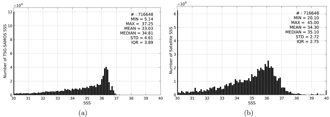
Figure 2: Histograms of SSS from TSG-SAMOS (a) and SMAP-L2-JPL-V4 (b) considering all match-up pairs per bins of 0.1 over the Mississippi river plume Pi-MEP region and for the full satellite product period.
