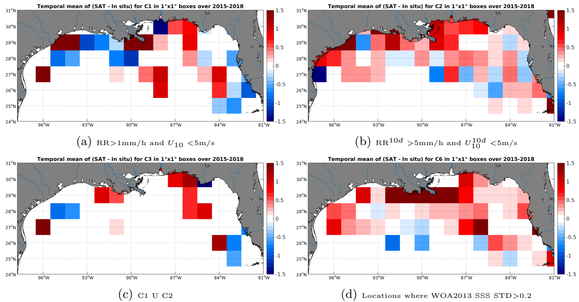
Figure 12: Temporal mean gridded over spatial boxes of size 1°x1° of \Delta SSS (SMAP-L2-JPL-V4 - TSG-SAMOS) for 4 different subdatasets corresponding to:RR>1mm/h and U_{10} < 5 m/s (a), RR^{10d} > 5 mm/h and U_{10}^{10d} < 5 m/s (b), C1 U C2 (c),Locations where WOA2013 SSS STD>0.2 (d).
