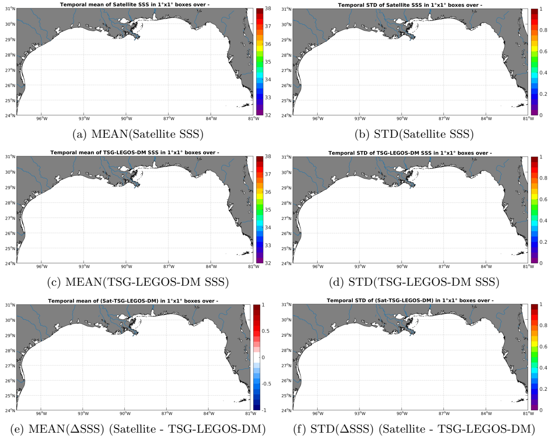
Figure 6: Temporal mean (left) and STD (right) of SSS from SMAP-L2-JPL-V4 (top), TSG-LEGOS-DM (middle), and of \Delta SSS (Satellite - TSG-LEGOS-DM). Only match-up pairs are used to generate these maps.
