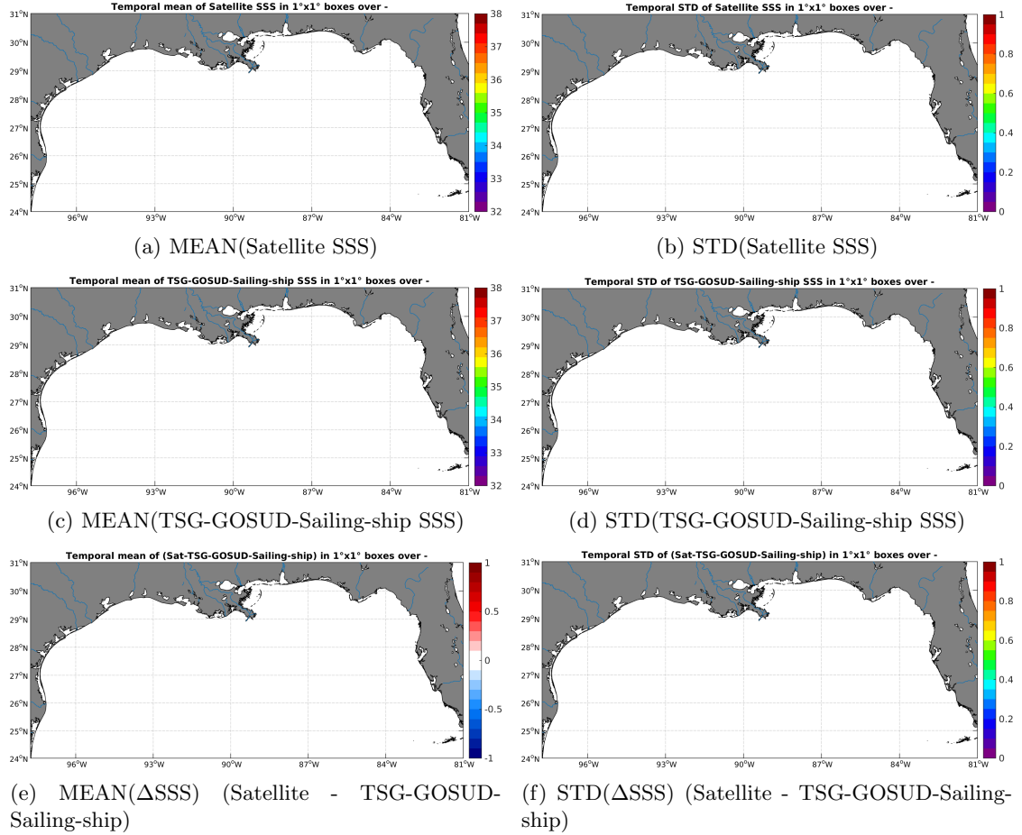
Figure 6: Temporal mean (left) and STD (right) of SSS from SMAP-L2-JPL-V4 (top), TSG-GOSUD-Sailing-ship (middle), and of \Delta\text{SSS} (Satellite - TSG-GOSUD-Sailing-ship). Only match-up pairs are used to generate these maps.
