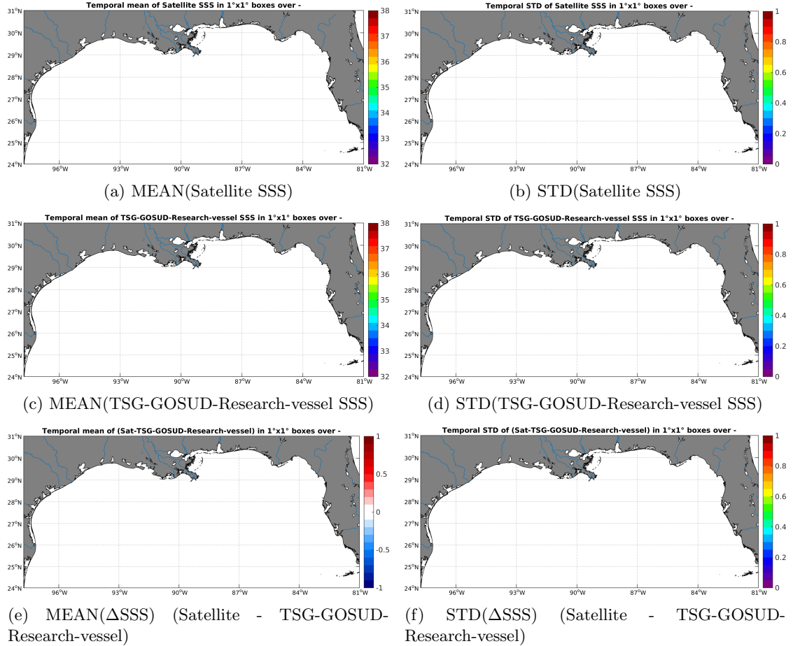
Figure 6: Temporal mean (left) and STD (right) of SSS from SMAP-L2-JPL-V4 (top), TSG-GOSUD-Research-vessel (middle), and of \Delta SSS (Satellite - TSG-GOSUD-Research-vessel). Only match-up pairs are used to generate these maps.
