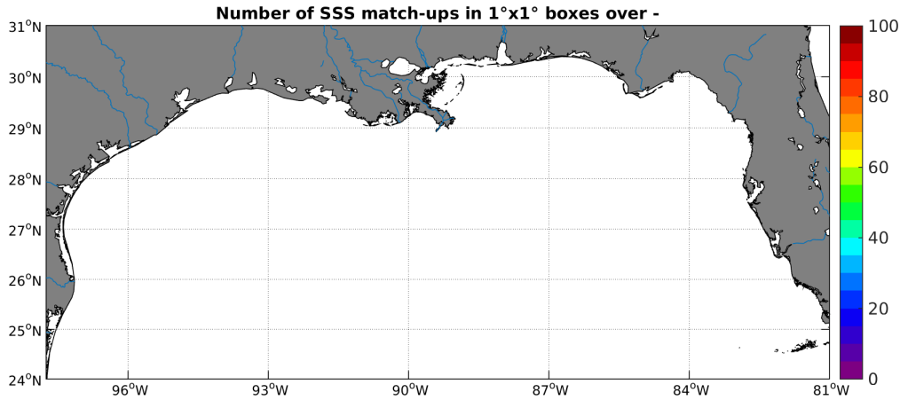
Figure 4: Number of SSS match-ups between Sea mammals SSS and the SMAP-L2-JPL-V4 SSS product for the Mississippi river plume Pi-MEP region over 1^\circ \times 1^\circ boxes and for the full satellite product period.
