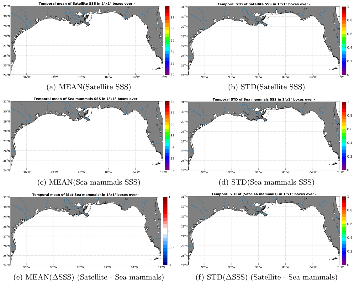
Figure 6: Temporal mean (left) and STD (right) of SSS from SMAP-L2-JPL-V4 (top), Sea mammals (middle), and of \Delta SSS (Satellite - Sea mammals). Only match-up pairs are used to generate these maps.
